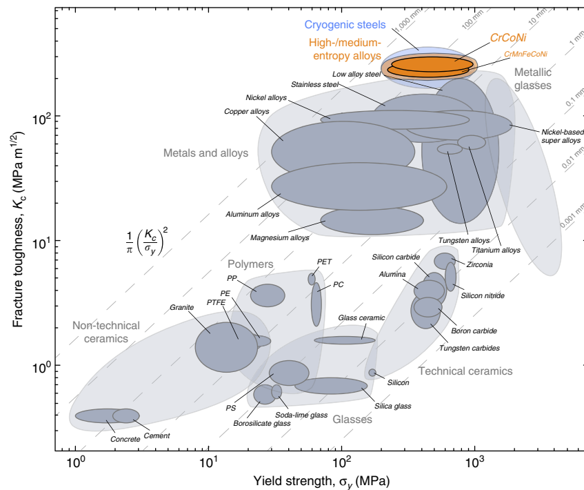
Figure 4 | Ashby map of fracture toughness versus yield strength for various classes of materials. The investigated medium-entropy alloy CrCoNi compares favourably with materials classes like metals and alloys and metallic glasses. Its combination of strength and toughness (that is damage tolerance) is comparable to cryogenic steels, for example, certain austenitic stainless steels 43–47 and high-Ni steels 48–51 , and exceeds all high- and medium-entropy alloys reported to date.
