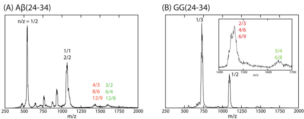
Figure 5. n-ESI-quadrupole mass spectra of (A) Aβ(24-34) and (B) GG(24-34). Each mass spectral peak is annotated with n/z ratio where n is oligomer number and z is charge. When multiple designations occur, they come from analysis of the ATD of that peak. The peptide concentration is 50 \mu M.
