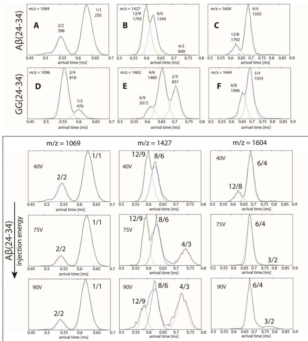
Figure 6. (Top panel) Representative arrival time distributions (ATDs) of the n/z = 1/1 , 4/3 and 3/2 peaks of Aβ(24-34), and 1/2 , 2/3 and 3/4 of its GG tandem version. The features in the ATDs of the low charge state peaks are assigned based on injection energy studies. Each feature is annotated with n/z ratio and experimental cross section \sigma in Å 2 . The narrow dashed lines are the peak shapes predicted for a single conformer of the cross sections given in the Figure. The peptide concentration is 50 μM. (Bottom panel, in box) Representative ATDs illustrating the injection energy studies for Aβ(24-34).
