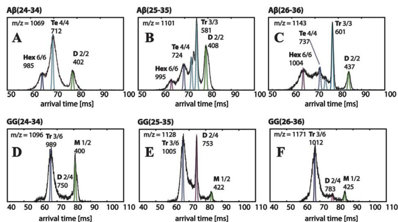
Figure 3. Representative arrival time distributions (ATDs) of the natural charge state (one charge per monomer) peaks of A \beta (24-34), A \beta (25-35), A \beta (26-36) and their GG versions obtained from instrument I. Each feature is labeled with oligomer size (M = monomer, D = dimer, Tr = trimer, Te = tetramer, Hex = hexamer), n/z ratio and experimental cross section \sigma in \text{\AA}^2 . The peptide concentration is 100 \mu\text{M} . The narrow dashed lines are the peak shapes predicted for a single conformer of the cross sections given in the Figure. The ATD features are broader than the predicted shape for a single conformer, suggesting there are multiple families of structures with similar cross sections. The cross sections listed above the peaks and in Table 2 correspond to these dotted line peaks.
