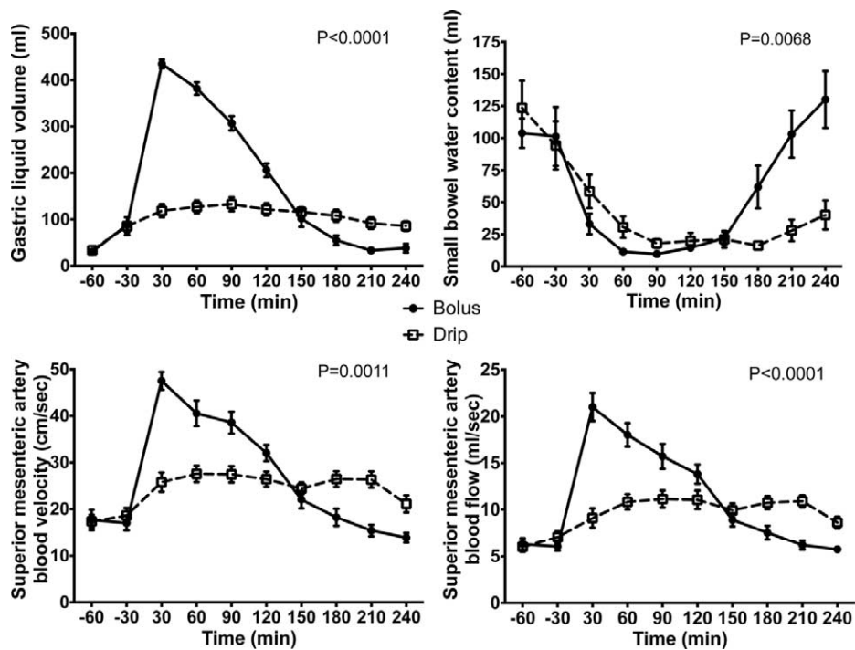
FIGURE 2. Changes in gastric liquid volume, small bowel water content, superior mesenteric artery blood velocity, and superior mesenteric artery blood flow after nasogastric infusion of 400 ml of Nestle Resource Energy over 4 hours (continuous) or 5 minutes (bolus). All values are mean \pm SEM. The P values are for the test of continuous drip versus bolus feeding using the analysis of variances and a repeated measures model.
