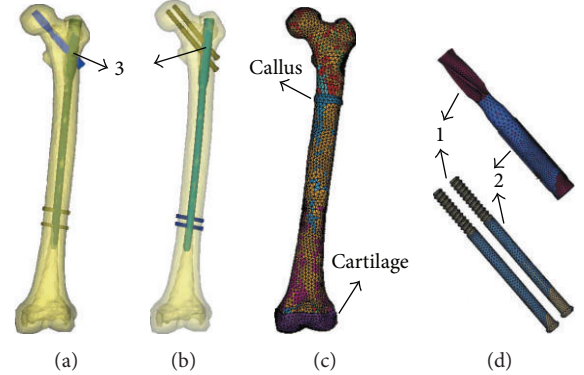
FIGURE 1: The finite element models (a, b) PFNA-II and A2FN implants fixing the femur models; (c) FE model of the elderly femur with the element-by-element material properties; (d) the femoral neck load carrier (PFNA-II blade/A2FN screws). Three different contact conditions in the bone-implant-construct (1 = contact elements, 2 = sharing common nodes, and 3 = coupling nodes' degree of freedom).
