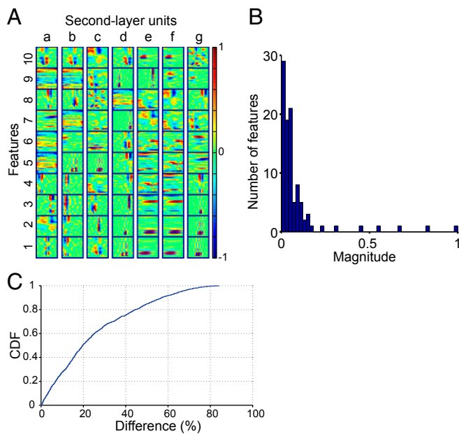
Fig. 6. Neural network trained on starling songs learns composite receptive fields. (A) Ten most active features for seven randomly chosen layer-2 units (a to g). (B) A histogram showing a distribution of the basis features' activities for one layer-2 unit. The absolute normalized magnitude is shown for comparison with the distributions of features' magnitudes in Figs. 2B and 5B. Note that most features are close to zero (lifetime sparseness) and that the most active features are of the same order of magnitude, as expected. (C) Cumulative density function (CDF) showing the percentage difference in the pair-wise magnitude between neighboring most active features of all layer-2 units. Ten largest basis features are selected for each layer-2 unit and sorted according to their activity (magnitude), then the percent difference is taken between the neighboring values.
