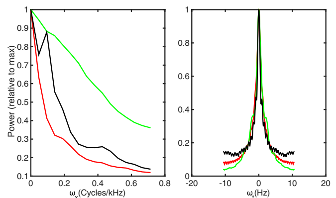
Fig. 3. Capturing the statistics of feature ensembles. Projections of modulation power spectra for starling songs (green), MNE features (red), and artificial neural network features (black) on spectral ( Left ) and temporal ( Right ) axes.
