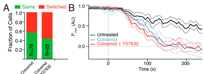
Fig. 6. MT disruption alters moesin polarization and disrupts memory. (A) Directional repolarization statistics for cells exposed to colcemid alone or colcemid and Y27632. (B) Average relaxation curves of moesin-mApple for untreated cells, cells exposed to colcemid and cells exposed to both colcemid and Y27632. Solid lines represent the average value across the population, dashed lines represent one SD.
