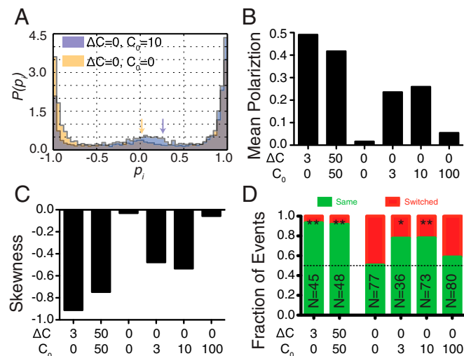
Fig. 2. Cells in uniform, nonzero concentrations exhibit a directional bias. (A) Histograms of instantaneous cell polarizations (PH-Akt) for cells in uniform concentrations of 0 nM (yellow) and 10 nM fMLP (blue). For the histograms shown all polarizations before the first depolarization of a cell were removed as described in the methods. Arrows designate the mean polarization. (B) Mean values for histograms of instantaneous polarizations. (C) Skewness of histograms of instantaneous polarizations (SI Experimental Procedures ). (D) Statistics of repolarization direction. Green represents the percentage of events for which a cell repolarized in the same direction as before depolarization. Red represents the percentage of events for which a cell switched direction.
