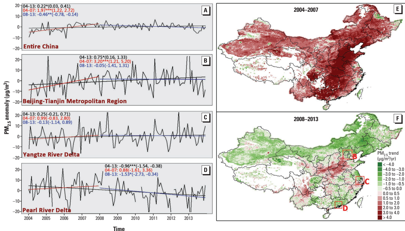
Figure 7. Time series of monthly, satellite-derived PM 2.5 anomaly (μg/m 3 ) for all of China (A), the Beijing-Tianjin metropolitan region (B), the Yangtze River delta (C), and the Pearl River delta (D); and spatial distribution of PM 2.5 trends for 2004–2007 (E) and 2008–2013 (F). The white areas in (E) and (F) indicate missing data. The black lines in A–D denote the PM 2.5 trends for 2004–2013, the red lines represent the trends for 2004–2007, and the blue lines represent the trends for 2008–2013. The PM 2.5 trends (μg/m 3 per year), 95% confidence intervals (CIs) in parentheses (μg/m 3 per year), and significance levels (* p < 0.05 ; ** p < 0.01 ; *** p < 0.005 ) are also shown in A–D.
