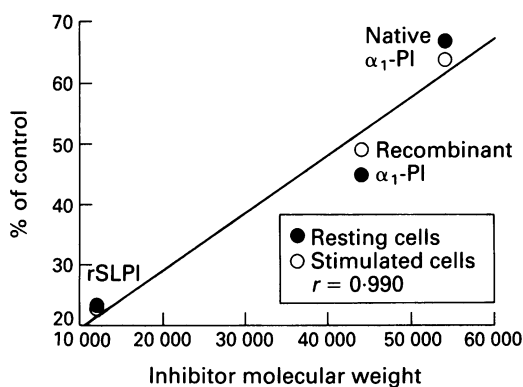
Figure 1 Relation between the molecular size of recombinant SLPI, recombinant \alpha_1 -PI and native \alpha_1 -PI and their ability to inhibit fibronectin degradation by resting and stimulated neutrophils adherent to fibronectin. Data are presented as percentage of control values in the absence of inhibitor.
