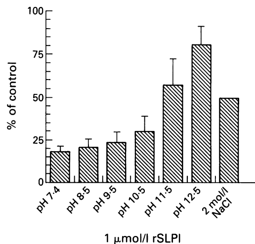
Figure 3 Effect of pretreating fibronectin wells with 1 μmol/l rSLPI in buffer of increasing pH (pH 7.4 to 12.5) or 2 mol/l NaCl solution on neutrophil degradation of fibronectin. The rSLPI was incubated with the fibronectin for one hour followed by washing and restoration of neutral pH before the addition of neutrophils. Data are presented as a percentage of the control values, control being neutrophil degradation of fibronectin following pretreatment of fibronectin with buffer alone. Each histogram represents the mean (SE) of four experiments.
