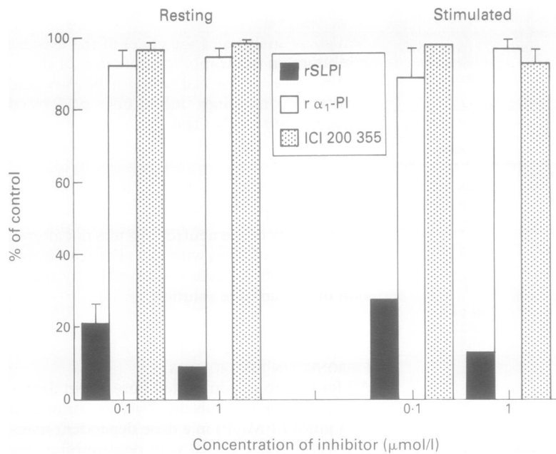
Figure 2 Effect of 0.1 μmol/l and 1.0 μmol/l rSLPI, rα 1 -PI, and ICI 200 355 pretreatment of fibronectin (followed by extensive washing) on fibronectin degradation by resting cells and cells stimulated with 1 μmol/l FMLP. Data are expressed as a percentage of control values where control is the amount of fibronectin degradation by neutrophils in wells pretreated with RPMI medium. Each histogram represents the mean (SE) of three replicates.
