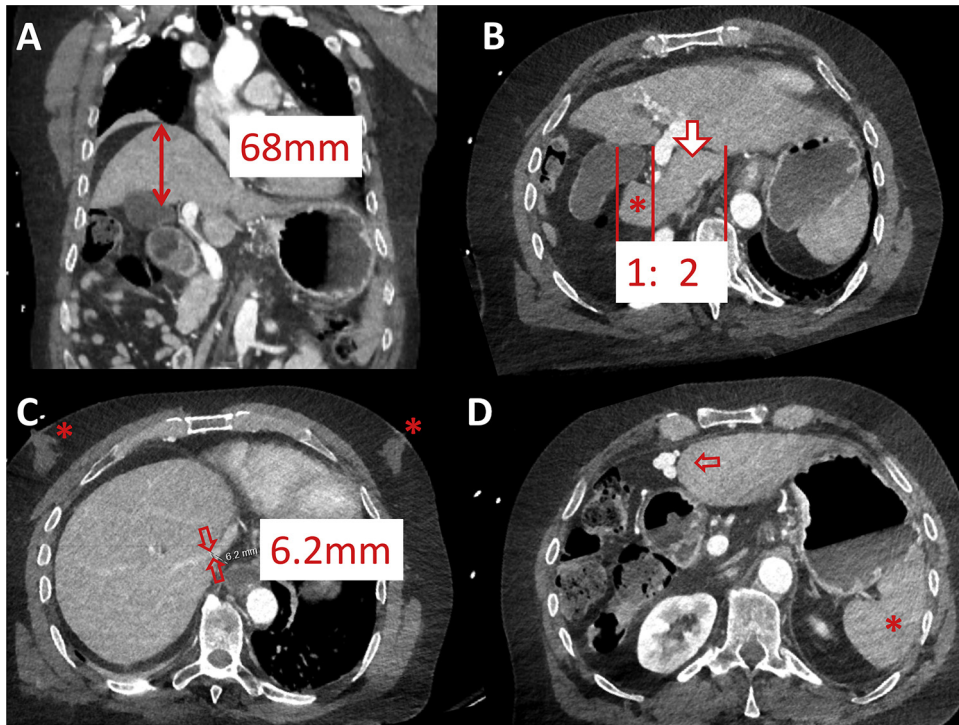
Fig. 5. (A, B) CT of liver cirrhosis with right lobe atrophy and left lobe hypertrophy complex with a caudate (arrow) to right (asterisk) lobe ratio >1. (C) Right vein diameter <7 mm due to compression of cirrhotic liver parenchyma; note additional gynecomasty (asterisk). (D) Signs of portal venous hypertension with recanalisation of umbilical vein and therefore no extensive splenomegaly (asterisk).
