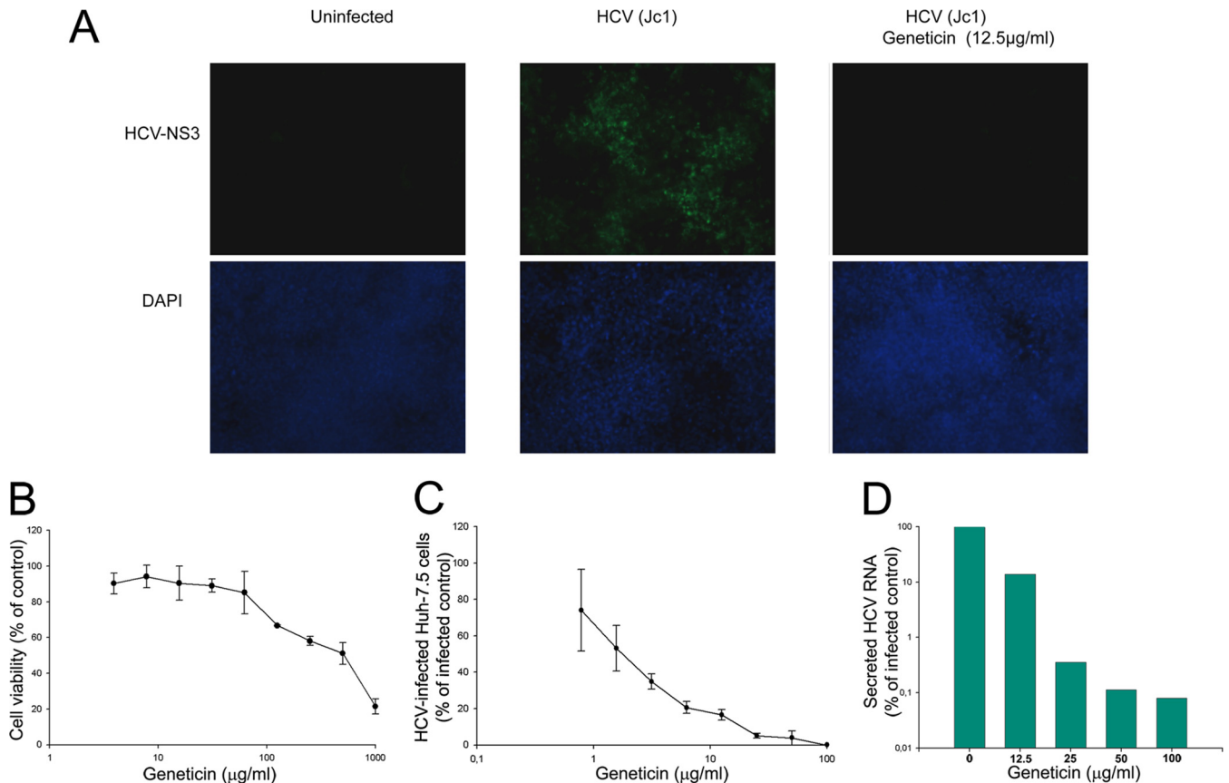
FIG 5 Geneticin inhibits the spread of HCV Jc1 infection in Huh7.5 cells. (A) (Top) Representative visualization of HCV NS3 protein in Huh7.5 cells after 4 days of infection in the presence or absence of 12.5 µg/ml Geneticin. (Bottom) The background cell density was visualized using DAPI (4',6-diamidino-2-phenylindole). (B) Cell viability in the presence of Geneticin. (C) NS3-stained cells in each focus were counted and quantified for spread of viral infection in the absence and presence of different concentrations of Geneticin. The values represent average results obtained from three independent experiments with EC_{50} s of ~2 µg/ml. (D) Virus yields in culture media as detected by qRT-PCR of culture medium at 96 h postinfection and then normalized to a percentage of the infected control ( EC_{50} s, ~12 µg/ml). The values represent averages and standard deviations of results from three independent experiments. The toxicity of Geneticin in Huh7.5 cells was detected using the alamarBlue assay (see Materials and Methods) ( LD_{50} , ~530 µg/ml).
