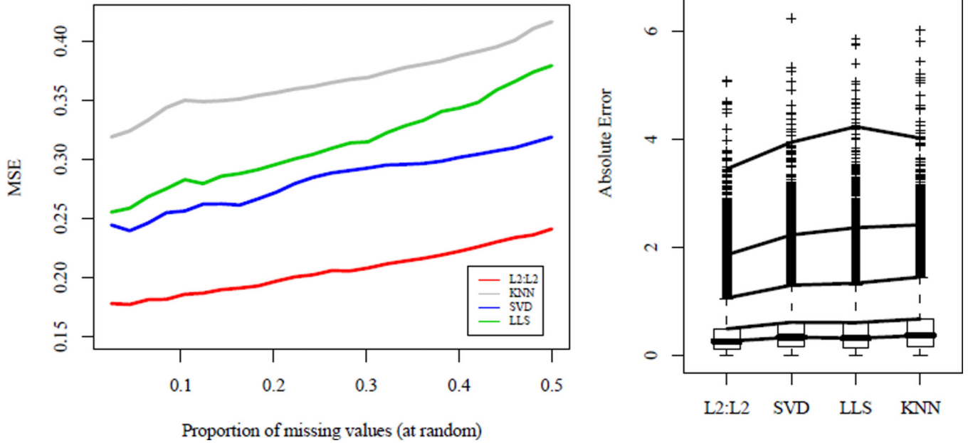
Fig 2. Left: Comparison of MSE for imputation methods on kidney cancer microarray data with different proportions of missing values. Genes in which all samples are observed are taken with values deleted at random. TRCMAimpute, L_2 : L_2 and common imputation methods KNNimpute, SVDimpute and LLSimpute are compared with all parameters chosen by 5-fold cross-validation. Cross-validation chose to penalize only the arrays for the one-step approximation algorithm, TRCMAimpute. Right: Boxplots of individual absolute errors for various imputation methods. Genes in which all samples are observed were taken and deleted in the same pattern as a random gene in the original dataset. Lines are drawn at the 50%, 75%, 95%, 99%, and 99.9% quantiles. TRCMAimpute, L_2 : L_2 has a mean absolute error of 0.37 and has lower errors at every quantile than its closest competitor, SVDimpute which has a mean absolute error of 0.46.
