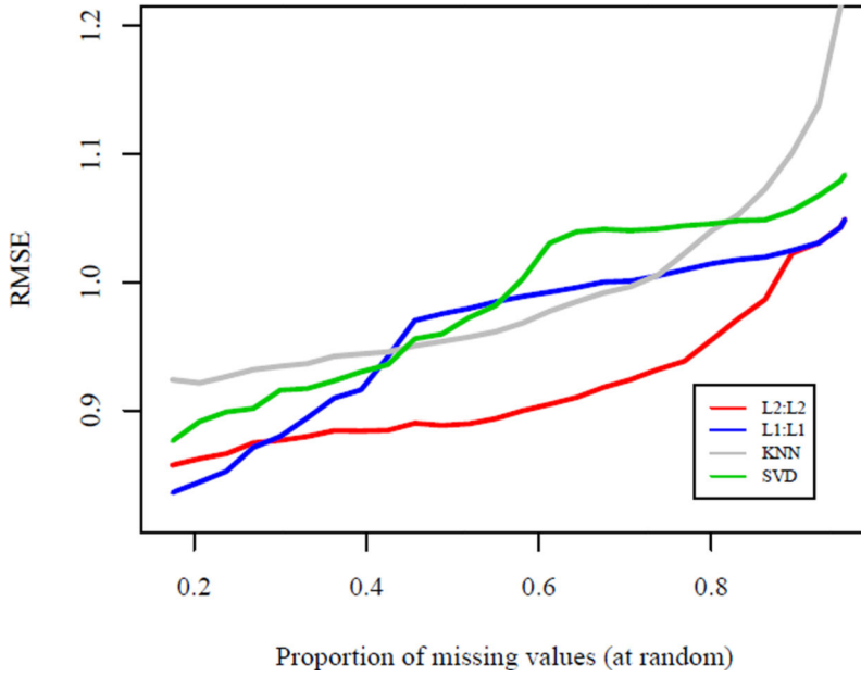
Fig 3. Left: Comparison of the root MSE (RMSE) for a subset of the Netflix data for TRCMAimpute, L_2 : L_2 and L_1 : L_1 , to KNNimpute and SVDimpute. A dense subset was obtained by ranking the movies and customers in terms of number of ratings and taking the top 250 movies and 250 customers. This subset has around 12% missing and additional values were deleted at random, up to 95%. With 95% missing, the RMSE of TRCMAimpute is 1.049 compared to 1.084 of the SVD and 1.354 using the movie averages. Right: Boxplots of absolute errors for the dense subset with missing entries in the pattern of the original data. Customers with at least one ranking out of the 250 movies were selected at random and entries were deleted according to these customers leaving 74% missing. Quantiles of the absolute errors are shown at 50%, 75%, 95%, 99%, and 99.9%. The RMSE of the methods are as follows L_2 : L_2 : 1.005, L_1 : L_1 : 1.029, SVD: 1.032, KNN: 1.184.
