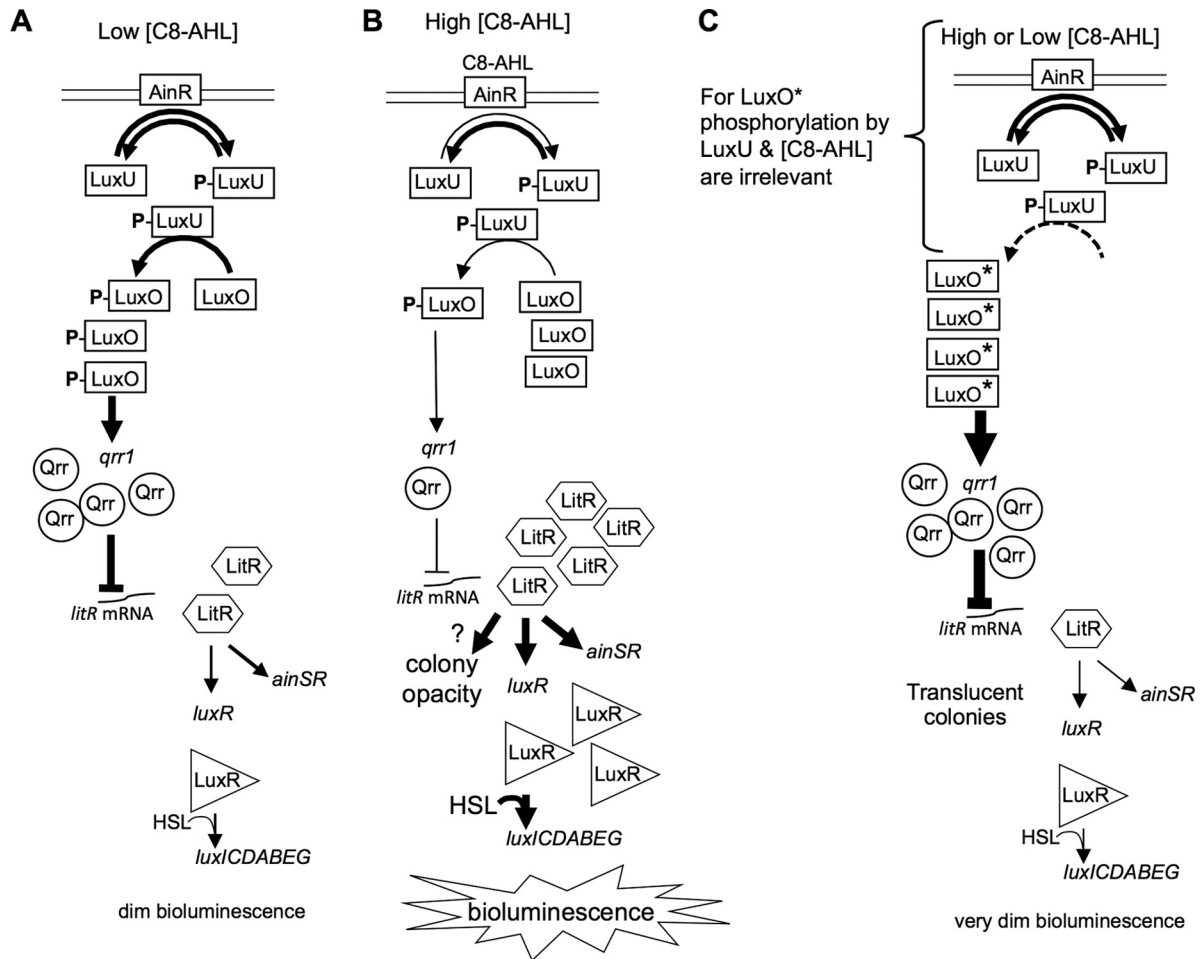
FIG 1 Model showing roles of Ain and LuxO in the pheromone regulatory circuit. The pheromone receptor AinR phosphorylates and dephosphorylates LuxU, which phosphorylates LuxO, stimulating it to activate transcription of qrr . The regulatory small RNA (sRNA) Qrr represses expression of the master regulator LitR. (A) At low C_8 -AHL levels, LuxO-P ultimately leads to relatively low LitR levels. (B) At high C_8 -AHL levels, binding of C_8 -AHL to AinR reduces its kinase activity, reducing the relative amounts of phosphorylated LuxU and LuxO, resulting in more LitR and induction of the LitR regulon, including luxR , bioluminescence, and ainSR . On plates, this induction also results in colony opacity through an unknown mechanism. (C) The activity of LuxO* does not require phosphorylation, although prior to this study, the effects of LuxU were untested. LuxO* essentially locks this circuit on “off,” and phenotypes resemble those at low C_8 -AHL levels. The colonies of luxO* mutants on plates remain translucent despite their high cell density.
