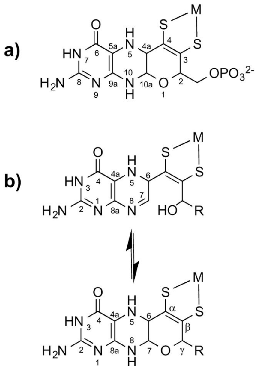
Figure 1. (a) Chemical structure and IUPAC numbering of MPT in the tricyclic pyranopterin form; (b) pyran cyclization equilibrium with the numbering system used in this paper. 4 It must be noted that, although the pterin IUPAC numbering system changes upon cyclization, the uncyclized numbering system (in (b), top structure) will be used throughout this paper for simplicity. M = Mo or W; R = phosphate or a dinucleotide.
