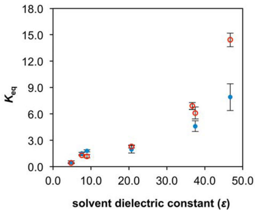
Figure 5. Plot of K_{eq} values versus solvent dielectric constant for 1 (open red circles) and 2 (blue dots).
