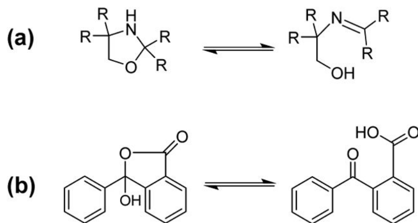
Figure 9. Examples of ring-chain tautomerism in (a) oxazolidines 32 and (b) o -benzoylbenzoic acids. 38
