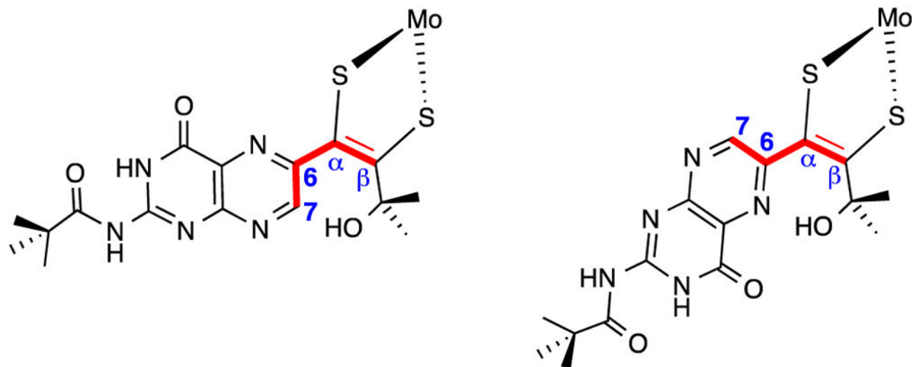
Figure 7. Structures illustrating the dihedral angle C7-C6-C\alpha-C\beta measured in the theoretical calculations; (left) for co-planar pterin and dithiolene groups, the dihedral angle C7-C6-C\alpha-C\beta is 0^\circ ; (right) for co-planar pterin and dithiolene groups, the dihedral angle C7-C6-C\alpha-C\beta is 180^\circ .
