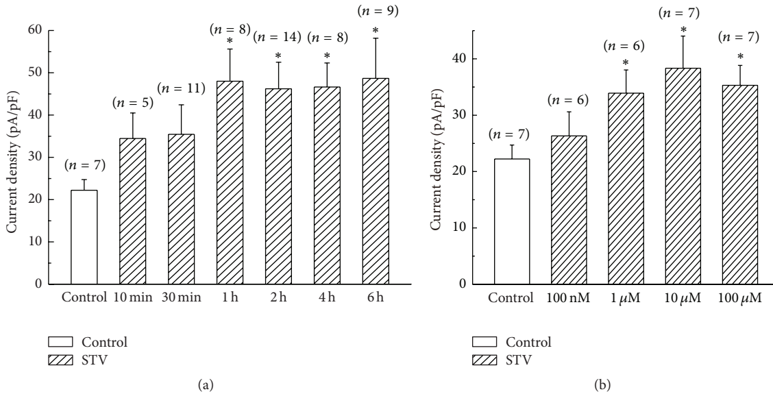
FIGURE 3: Time and concentration dependence of STV on pinacidil-activated K_{ATP} current. (a) The time dependence of STV-preincubation (10 \mu M) on pinacidil-induced K_{ATP} channel current. (b) The concentration dependence of STV on K_{ATP} current with incubation period of more than 1 hr. * means p < 0.05 .
