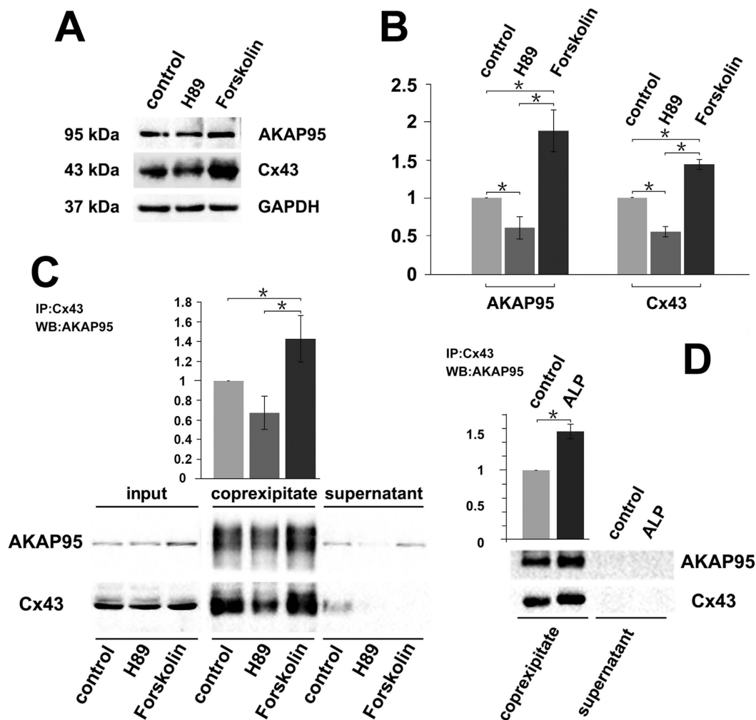
Figure 7. Binding between AKAP95 and Cx43 is affected by PKA activity. (A) Western blot examination of Cx43 and AKAP95 expression; GAPDH used as the internal reference. Each lane contains 30 \mu g of total proteins. The experiment was repeated three times. (B) Statistical data of AKAP95 and Cx43 expression levels in cells after H89 and Forskolin treatments (20 \mu M each). AKAP95 and Cx43 expression levels decreased in the H89 treatment ( p < 0.05 ) and increased in the Forskolin treatment compared to the control group ( p < 0.05 ). Images were acquired using the BioRad Chemi DOC XRS + Imaging System, and the gray value of protein bands was scanned using Image Lab5.0. The ratio of measurements of the treatment group to the control group was calculated by one-way analysis of variance in SPSS 21.0. (C) Western blot analysis of binding between AKAP95 and Cx43 in cells after H89 and Forskolin treatments. 500 \mu g of extracted total proteins was co-immunoprecipitated (Co-IP) with 3 \mu g of anti-Cx43 antibody. The Co-IP products were resuspended in an equal volume of loading buffer, and the supernatant was subjected to western blot with anti-Cx43 and anti-AKAP95 antibodies, and the grayscale value of the bands of the H89 and forskolin groups were compared with those of the control bands and the ratios were subjected to statistical analysis. (D) Western blot analysis of binding between AKAP95 and Cx43 after alkaline phosphatase (ALP) treatment. 500 \mu g of extracted total proteins was diluted to 0.2 \mu g/ \mu L with RIPA lysis buffer and split into two groups (500 \mu L each). The ALP treatment was performed following the manufacturer's instructions (see ALP treatment in M&M). The protein diluents were subjected to Co-IP with 1 \mu g of anti-Cx43 antibody, and the products were resuspended in an equal volume of loading buffer, and then were subjected to western blot analyzed with anti-Cx43 and anti-AKAP95 antibodies, the grayscale value of the bands of ALP treatment groups were compared with those of the control bands and the ratios were subjected to statistical analysis. Results showed that the binding capacity of Cx43 and AKAP95 was improved after ALP treatment. The experiment was repeated three times.
