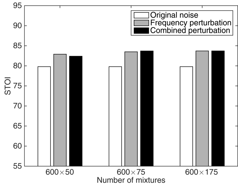
Figure 8. Average STOI (in %) of separated speech for six noises at -5 dB with respect to the number of training mixtures.
