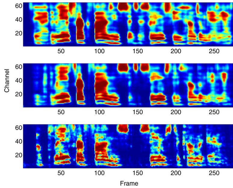
Figure 9. Mask comparisons. The top shows a ratio mask obtained from training on original noises, the middle shows a mask obtained from training on frequency perturbed noise, and the bottom shows the IRM.
