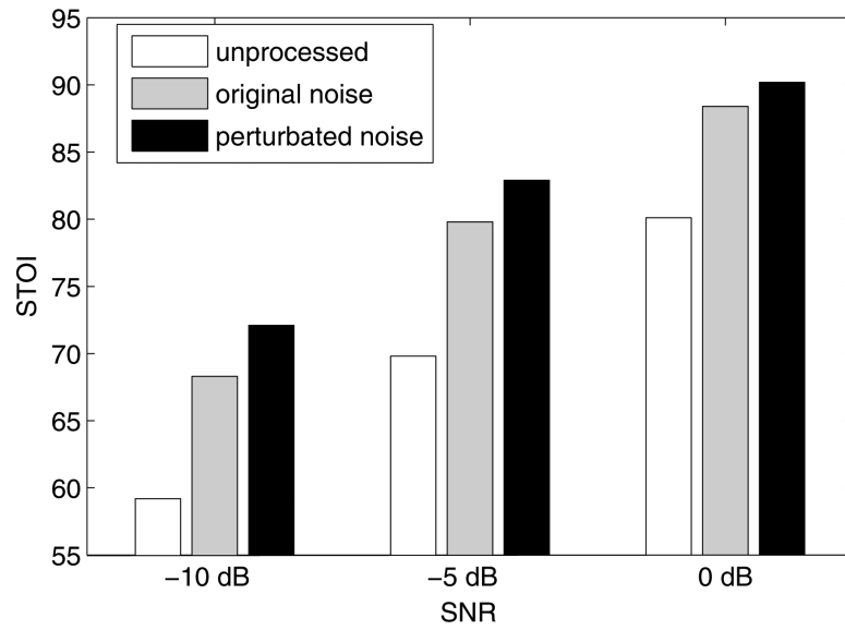
Figure 10. The effect of frequency perturbation in three SNR conditions. The average STOI scores (in %) across six noises are shown for unprocessed speech, separated speech by training on original noises, and separated speech by training on frequency perturbed noises.
