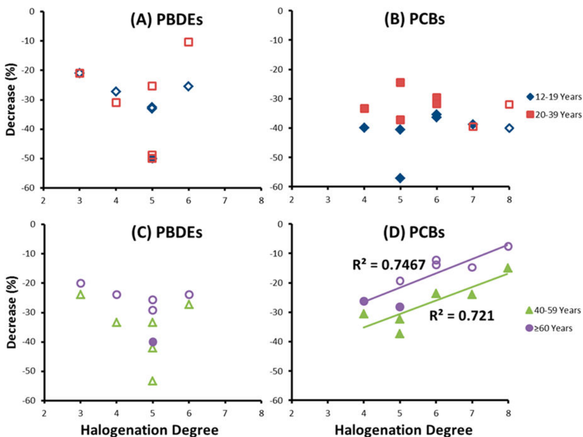
Figure 3. Percent decrease in arithmetic mean concentration of PCB and PBDE congeners by halogenation degree for four different age groups, from NHANES 2003/04 to 2007/08. Filed markers indicate differences in arithmetic mean for which the 95% CI did not overlap while nonfiled markers refer to comparison with overlap of 95% CI. Linear regression line has been drawn when the p -value for regression was <0.05 .
