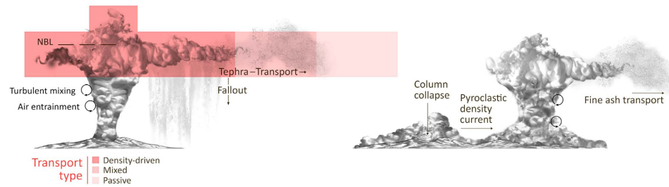
Figure 1. Schematic diagram (not to scale) of a super-eruption event with an initial (left) sustained Plinian phase followed by a column-collapse and large pyroclastic density currents eventually leading to co-ignimbrite plumes offset from the vent (right). Colour cells mark the extent of each transport regimes in the umbrella cloud.
