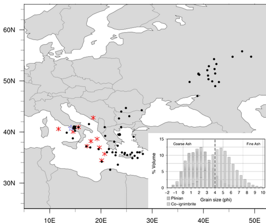
Figure 2. Map showing the location of the CI-caldera (star) and geological samples in dataset 1 (asterisks) and 2 (circles). The inset shows the reconstructed TGSD from dataset 1. The map was generated using the D3.js library.
