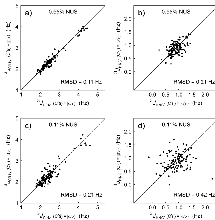
Fig. 3. Reproducibility of the duplicate measurements of ^3J couplings from the 4D NUS HACANH[C'] E.COSY spectrum of \alpha -synuclein. Comparisons of the duplicate ^3J_{C'Ha} measurements (see right panels of Fig. 2a) obtained when (a) using 0.55% NUS sampling and (c) 0.11% NUS sampling. Analogous comparisons of the two ^3J_{HNC'} measurements (see right two panels of Fig. 2c) obtained when using (b) 0.55% and (d) 0.11% NUS sampling.
