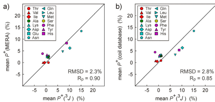
Fig. 6. Positive \phi angle propensity in \alpha -synuclein for different residue types. (a) Comparison of P^+ obtained from MERA analysis (lacking ^3J_{C^H\alpha} as input) with results of iterative analysis of ^3J_{C^H\alpha} , ^3J_{HNH\alpha} and ^3J_{C^C'} . (b) Comparison of P^+ obtained from iterative analysis of ^3J_{C^H\alpha} , ^3J_{HNH\alpha} and ^3J_{C^C'} with residue-type averaged P^+ values of the Mantyszov coil library. 14
