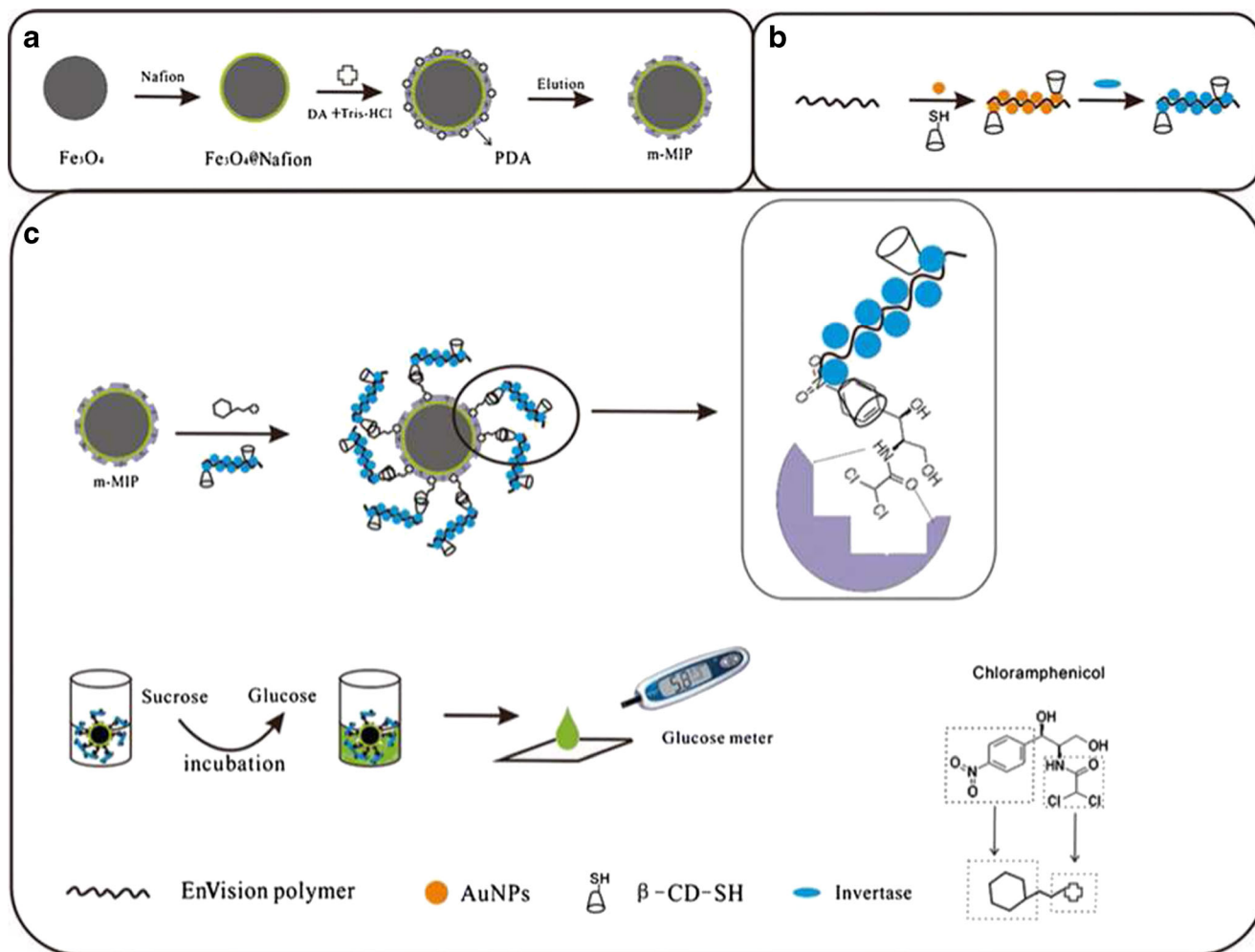
Fig. 13 a Preparation of magnetic molecularly imprinted polymers. b EnVision reagent (EV)-Au- \beta -cyclodextrin/invertase signal tag preparation. c Scheme for the sandwich assay [123]. With permission from Springer Science+Business Media: Analytical and Bioanalytical Chemistry. A portable and antibody-free sandwich assay for
