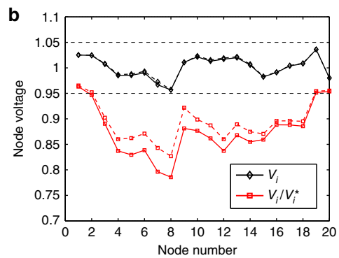
Figure 5 | Corrective action results for the reduced New England 39-node network. (a) Depiction of the reduced New England grid. Load nodes \{1, \dots, 30\} are red circles, while generators \{31, \dots, 39\} are green squares. Shunt capacitors are present at all load nodes, but shown explicitly at nodes 7, 8 and 9. (b) Results of corrective action study. Voltage profile V_i (black) and scaled voltages V_i/V_i^* (red), before (solid) and after (dashed) corrective action. All voltages were scaled by the grid’s base voltage V_{base} = 345 kV. Horizontal dashed lines are operational limits for V_i of \pm 5\% from base voltage. For clarity only nodes \{1, \dots, 20\} are plotted. Map by freevectormaps.com.
