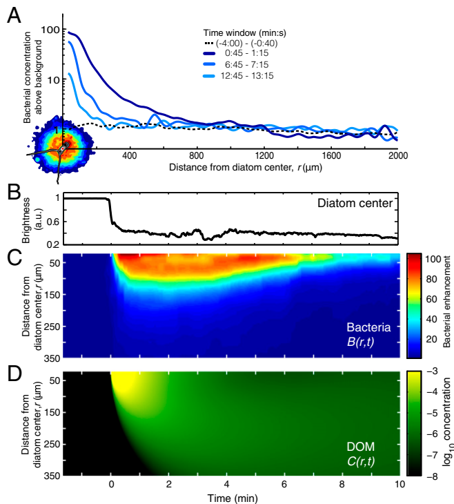
Fig. 2. Chemotactic accumulation in the phycosphere lasts \sim 10 min and extends \sim 2 mm from the diatom. All panels (A–D) show results for a prototypical radially symmetric cluster in response to lysis of a single C. affinis diatom. (A) Bacterial concentration above background as a function of distance from the diatom center, r , for three 30-s time windows after lysis. The prelysis background is also shown. An image of the lysed diatom (bottom left) shows relative bacterial concentration (color contours) at peak accumulation ( t = 1 min), with the same scale as the x axis. (B) Brightness of the diatom center (in arbitrary units) showing the moment at which lysis occurred, t = 0 . (C) Bacterial enhancement relative to the background concentration, B(r,t) . (D) Relative concentration of the effective chemoattractant as a function of distance and time, C(r,t) , determined from a mathematical simulation.
