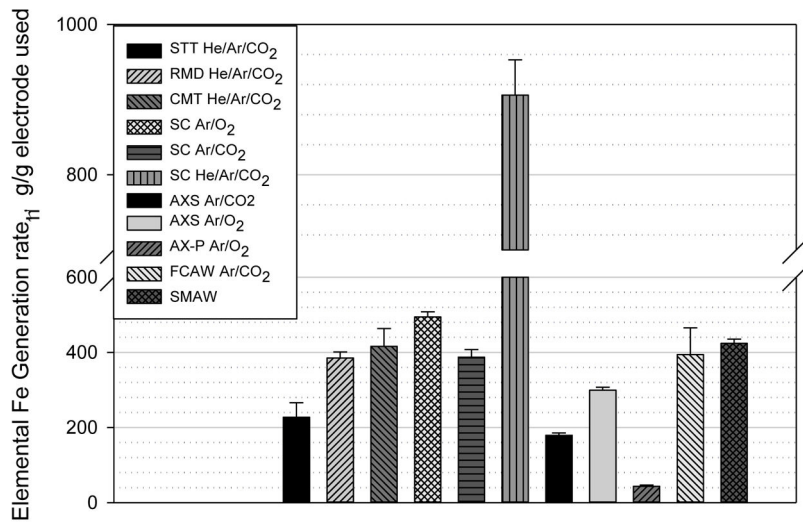
Figure 9. Elemental Fe generation rates for 11 processes, expressed as µg Fe per g of electrode consumed.
