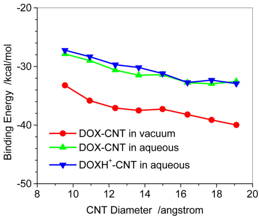
Fig. 4. Binding energies of DOX-loaded on outer surface of CNT with respect to CNT diameter with PM6-DH2method.
