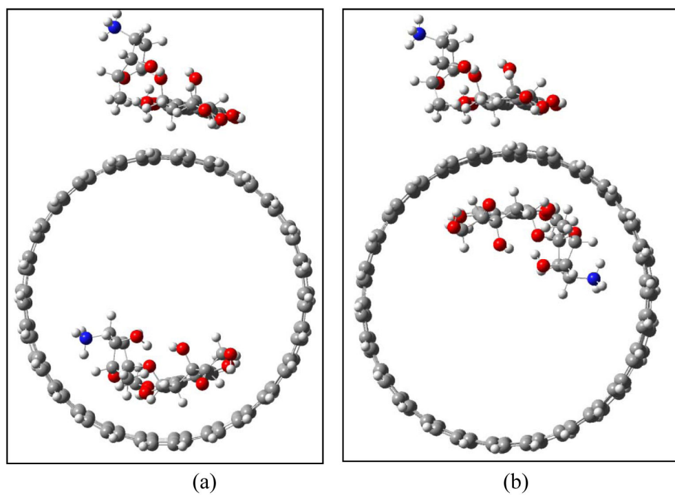
Figure 12. Mutual influence of adsorption and encapsulation of DOXH + -CNT(13,13) in the case of rather separated (a), and in the case of neighbor (b).
