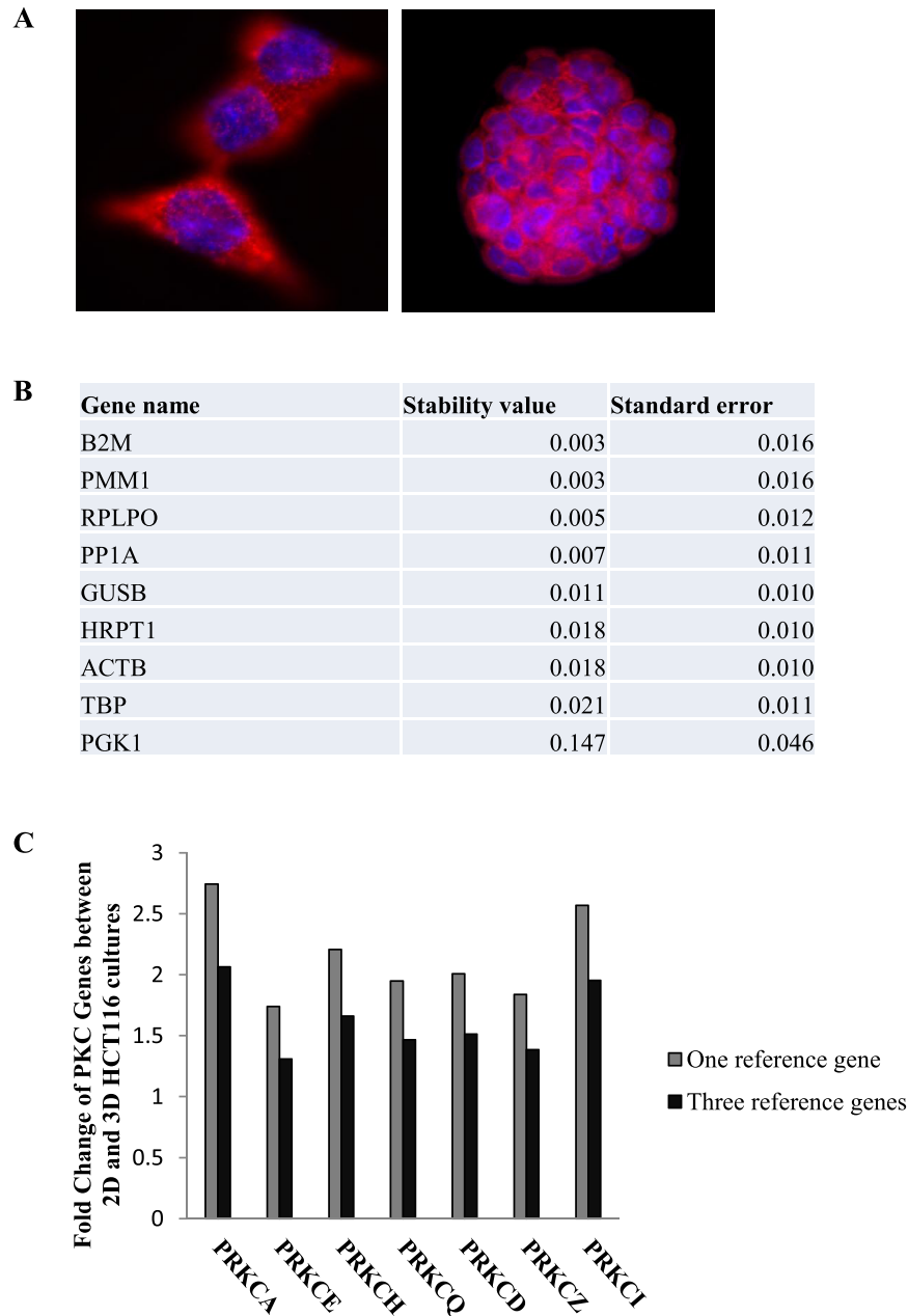
Figure 1. Reference genes in 2-dimensional and 3-dimensional HCT116 cultures. The stability of the nine candidate reference genes between 2D and 3D HCT116 cultures was analysed using NormFinder. (A) Immunofluorescence images of HCT116 cells in 2D (100X) ( left panel ) and 3D ( right panel ) cell cultures (63X). (B) Table displaying the stability levels of the nine candidate reference genes between the 2D and 3D cultures. (C) Graph representing the fold change of PKC coding genes in 3D cultures compared to 2D cultures when using one reference gene (B2M) versus three reference genes (B2M, PMM1 and RPLPO).
