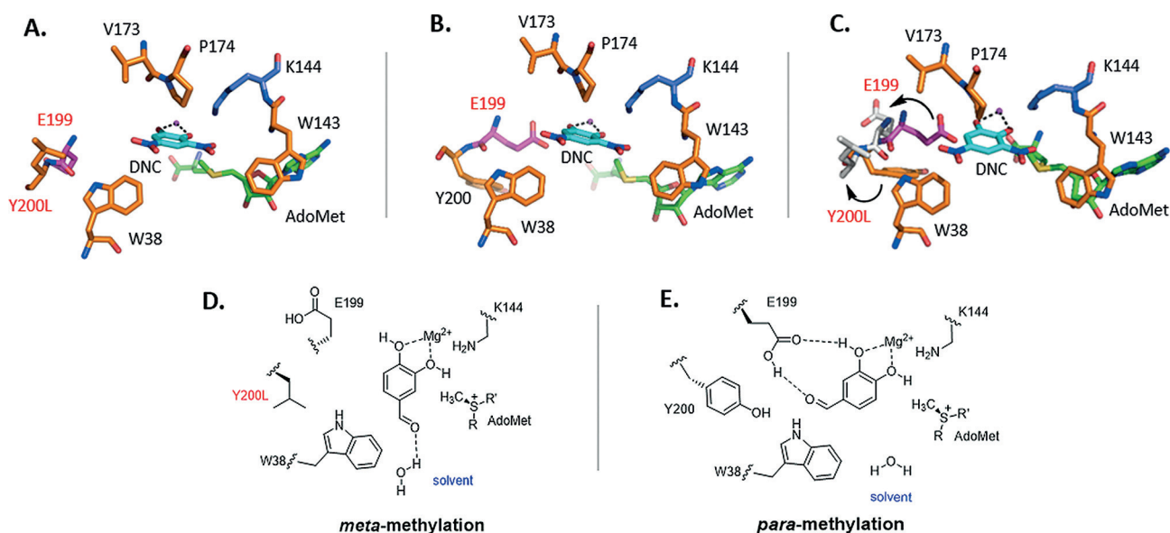
Figure 3. Crystal structures of COMT and proposed substrate binding modes for para - and meta -methylation. Mg^{2+} (magenta sphere) is shown coordinated (dashed lines) to the catechol hydroxy groups. A) COMT mutant Y200L complexed with DNC, showing the Y200L mutation that causes the adjacent E199 residue to flip out of the active site and lose contact with the catechol. B) Crystal structure of WT COMT monomer complexed with DNC (PDB ID: 1VID), with E199 in close proximity to the R group of bound substrates. C) Overlay of the Y200L and WT structures, showing the altered positions of Y200L and E199 in the mutant (grey). D) Substrate orientation for meta -methylation in Y200L. With E199 unable to hydrogen bond with the substrate aldehyde, the aldehyde group preferentially associates with the solvent, which positions the meta -hydroxy group adjacent to the AdoMet sulphonium centre. E) Substrate orientation for para -methylation in WT COMT, with the substrate aldehyde hydrogen bonding with E199, thereby orientating the catechol ring such that the para -hydroxy group is presented to AdoMet.
