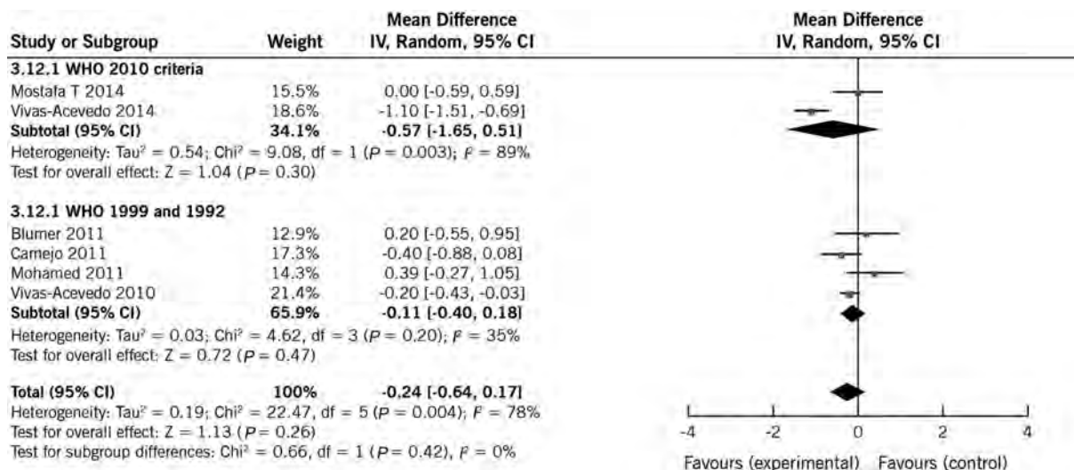
Figure 2: Forest plot showing the effect of varicocele on semen volume, including subgroup analyses according to different WHO criteria.
