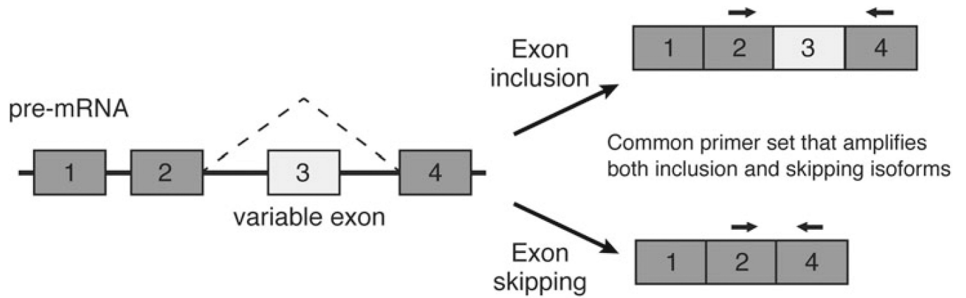
Fig. 2. Semi-quantitative PCR for examination of exon skipping. A schematic is shown depicting a hypothetical four-exon gene with variable exon 3 undergoing alternative splicing. The paired arrows indicate primer sets that flank the variable exon 3 and thus amplify both variable exon-inclusion and skipping isoforms from a cDNA template. The different splice isoforms can be distinguished by size using semi-quantitative PCR and electrophoresis
