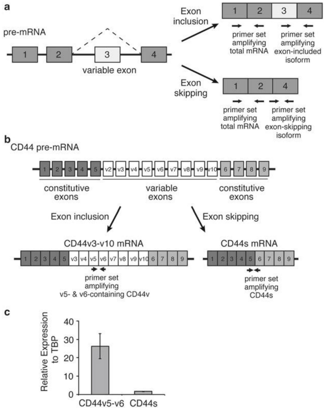
Fig. 1. Characterization of alternative splicing by qRT-PCR. (a) A schematic illustrating a hypothetical four-exon gene with a variable exon 3 that undergoes exon-inclusion or exon-skipping. Three primer sets for qPCR indicated by the paired arrows are designed to amplify the total mRNA, the variable exon 3 inclusion isoform, or the exon-skipping isoform. (b) A schematic depicting the exon structure of the transmembrane protein CD44, with the nine constitutive and nine variable exons labeled. CD44v3-v10 and CD44s are predominant splice isoforms and are depicted. Paired arrows indicate primer sets to amplify CD44v v5-
