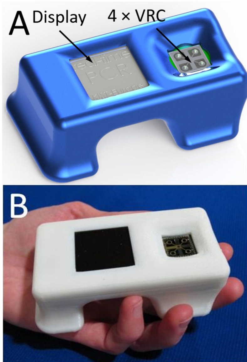
Figure 1. (A) CAD design drawing of the hand held PCR. The illustration shows a display with a compartment accommodating 4 samples in VRC form. (B) Fabricated and assembled complete real-time PCR device packaged within a 3D printed casing.
