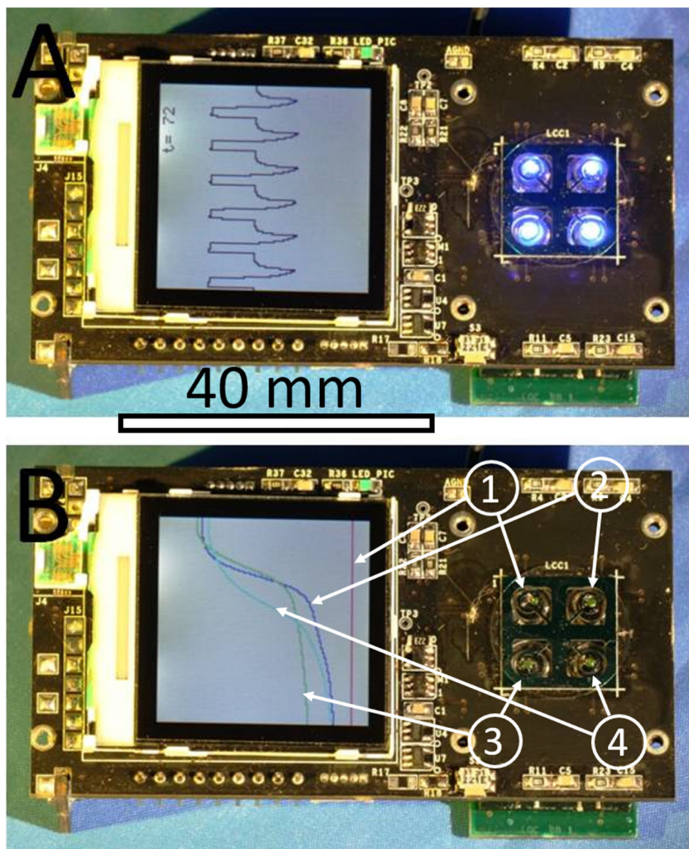
Figure 4. (A) An assembled PCR system with four VRCs, each consisting of a \approx 0.5 \mu\text{L} sized sample covered with \approx 1.5 \mu\text{L} of M5904 mineral oil, showing the PCR temperature profile (protocol) within the LCD display. The device size is 82 \text{ mm} \times 45 \text{ mm} \times 20 \text{ mm} (length, width and height). Scale bar is 40 mm. The protocol started by a “hot start” to activate the polymerase enzyme for \approx 10 \text{ min} at \approx 95 \text{ }^\circ\text{C} , followed by 40 cycles of PCR amplifications. Each amplification cycle consisted of 3 steps. First, denaturation for \approx 10 \text{ s} at \approx 95 \text{ }^\circ\text{C} , then annealing for \approx 10 \text{ s} at \approx 50 \text{ }^\circ\text{C} and the last step was extension for \approx 15 \text{ s} at \approx 68 \text{ }^\circ\text{C} (instead of typical \approx 72 \text{ }^\circ\text{C} ), during which fluorescence was measured. The LCD display shows 6 cycles. At the completion of each PCR amplification cycle, fluorescence amplitude at each spot was calculated and amplification curves were plotted in (B). We placed NTC at position 1, low concentration of complementary DNA (cDNA) from H7N9 HA gene at position 3,
