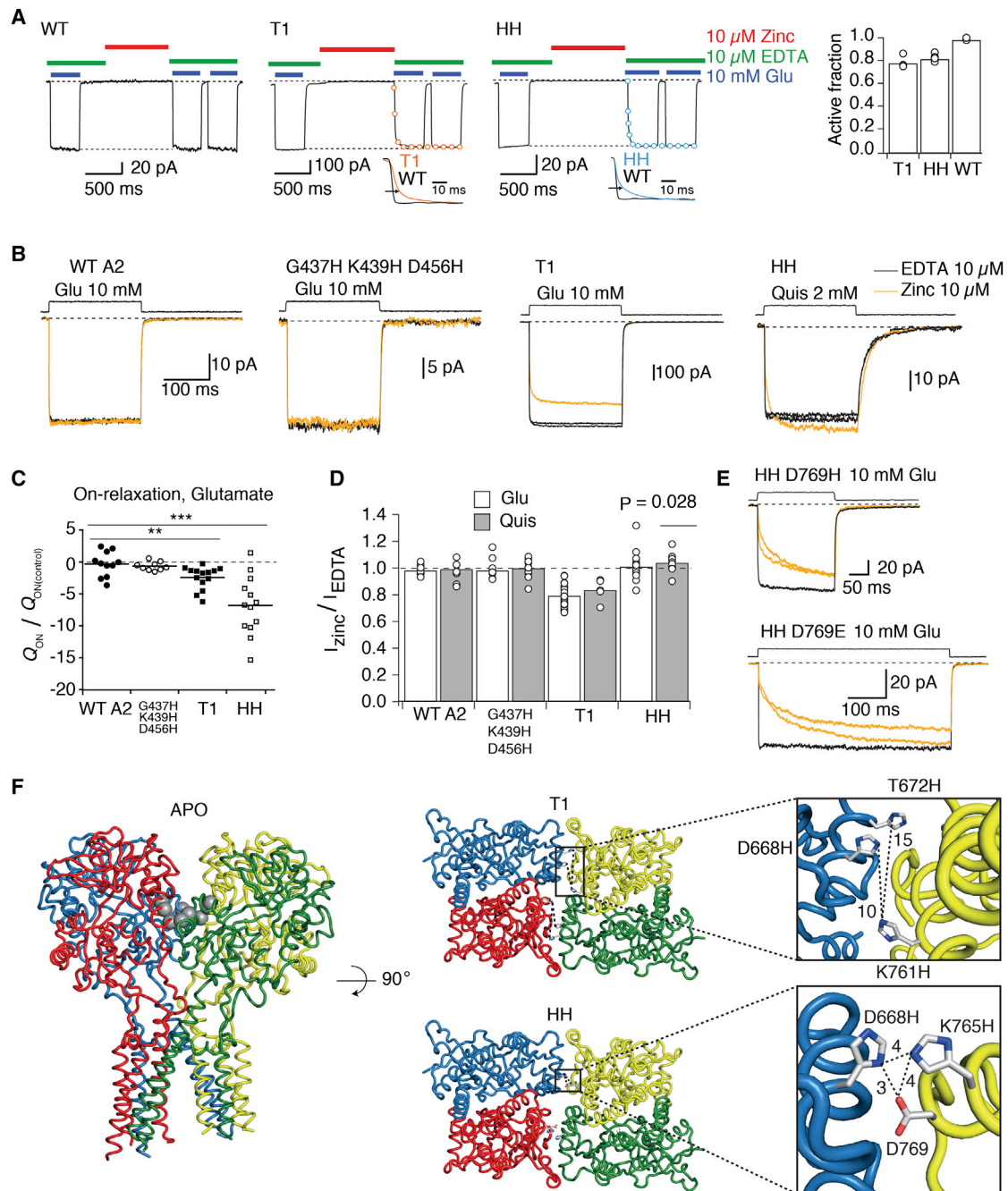
FIGURE 5 Apo state trapping. (A) WT receptors are unaffected by 1 s exposure to zinc (10 \mu M) in the absence of any ligand, but both, the T1 and HH mutants exhibit slower on-relaxation upon jump into (zinc-free) glutamate. For both mutants, the on-relaxation contained two components: \tau_1 = 5 \pm 0.5 ms and \tau_2 = 91 \pm 12 ms ( n = 4 patches) for T1 and \tau_1 = 9 \pm 4 ms and \tau_2 = 90 \pm 12 ms ( n = 4 ) for HH. The faster component reflects the solution exchange, and the slower component corresponds to relaxation from zinc trapping, i.e., lifetime of the bridges formed in zinc. The bar graph shows the residual active current after exposure in the apo state to 10 \mu M zinc. (B) Traces showing WT and mutant receptors jumped into 10 mM glutamate (Glu) or 2 mM quisqualate (Quis) in the absence (10 \mu M EDTA, black traces) or presence of zinc (10 \mu M, orange traces) with zinc or EDTA present throughout the recording. CTZ (100 \mu M) was also present throughout the recording to block desensitization. The effects of zinc are reversible as shown by alternating jumps between zinc-containing and zinc-free solutions. (C) Summary of the effects of zinc on the on-relaxation. For each patch, traces in EDTA and zinc were separately averaged and normalized to their peak. Their difference trace was then integrated to obtain the cumulative difference in charge ( Q ). We determined the average variability of Q_{ON} within groups ( Q_{ON(\text{control})} ) to control for the inherent variability. Q_{ON} was then normalized by Q_{ON(\text{control})} . Q_{ON} was measured 100 ms after the start of the agonist pulse. The trapping mutants, T1 and HH both showed slower on-relaxation in zinc, and thus a deficit of charge during the rise to the peak current, in both glutamate and quisqualate (not shown) *** p < 0.001 , * p < 0.05 . (D) Plot summarizing the effects of zinc on the steady-state current in glutamate (white bars) and quisqualate (gray bars) for T1, HH, and the controls (WT and CA-HHH). The steady-state current is the average current of the last 30 ms of the agonist pulse. (E) The HH D769H mutant showed a similar functional profile to the T1 mutant when equilibrated in 10 \mu M zinc
