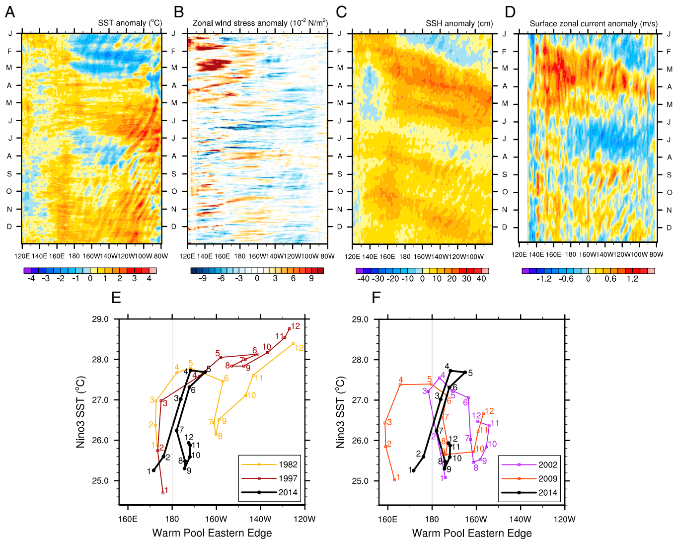
Fig. 2. Spatiotemporal evolution of the 2014 El Niño. (A–D) Hovmöller diagrams for anomalies in (A) SST, (B) zonal wind stress, (C) SSH, and (D) surface zonal currents in the equatorial Pacific. Time goes downward. The SSH and surface velocity plots highlight the eastward propagating downwelling Kelvin waves, especially pronounced early in the year, and a strong upwelling Kelvin wave midyear. (E and F) El Niño development in 2014 (black line) compared with several historical (E) EP and (F) CP events. The diagrams show the position of the Warm Pool Eastern Edge (degrees of longitude) vs. the Niño3 SST (degrees Celsius) for different months of the year. The Warm Pool Eastern Edge is defined as the position of the 29 °C isotherm at the equator. Numbers indicate monthly averages (1, January; 2, February, etc.). The light vertical line marks the Dateline. In 2014, both the warm pool displacement and Niño3 SST anomalies were exceptionally large during May (month 5), were similar to those in 1997 and 1982 (the strongest events of the 20th century), and then, rapidly decreased by August (month 8).
