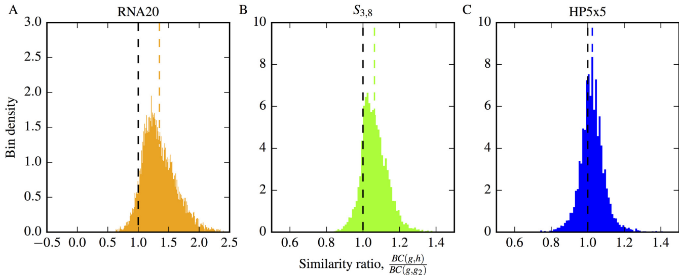
Fig 7. Non-neutral local mutational neighbourhood correlations result in mutational neighbourhoods of neutral neighbours being more similar than randomly selected neutral pairs. We present results for the three GP maps: A) RNA20, B) S_{3,8} and C) HP5x5. Using the ratio of Bhattacharyya coefficients defined in Eq (10), we show that neutral neighbours ( g and h ) have a closer phenotype probability distribution than a randomly chosen neutral pair ( g and g_2 ). This is seen through the ratio being skewed with a mean (coloured vertical dashed lines) larger than unity (black vertical dashed lines). The standard error on this mean is negligible compared to the distance of the mean from one.
