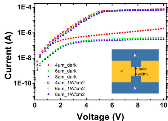
Figure 3. SLOT I-V Curve Measurement. Current-voltage characteristics are measured based on a rectangular-shaped phototransistor test structure. NPN phototransistors of three different base widths, 4 \mu\text{m} , 6 \mu\text{m} , and 8 \mu\text{m} , were tested. Photocurrent is measured under the illumination of a 532 nm green laser beam at an intensity of 1 W/cm 2 . The phototransistor with a 4 \mu\text{m} base width gives a higher photocurrent than others, but comes with a higher dark current too. In SLOT devices, base widths between 3.5 \mu\text{m} to 4 \mu\text{m} are typically used. For base width shorter than 3 \mu\text{m} , dark current becomes too high and affects the self-locking function.
