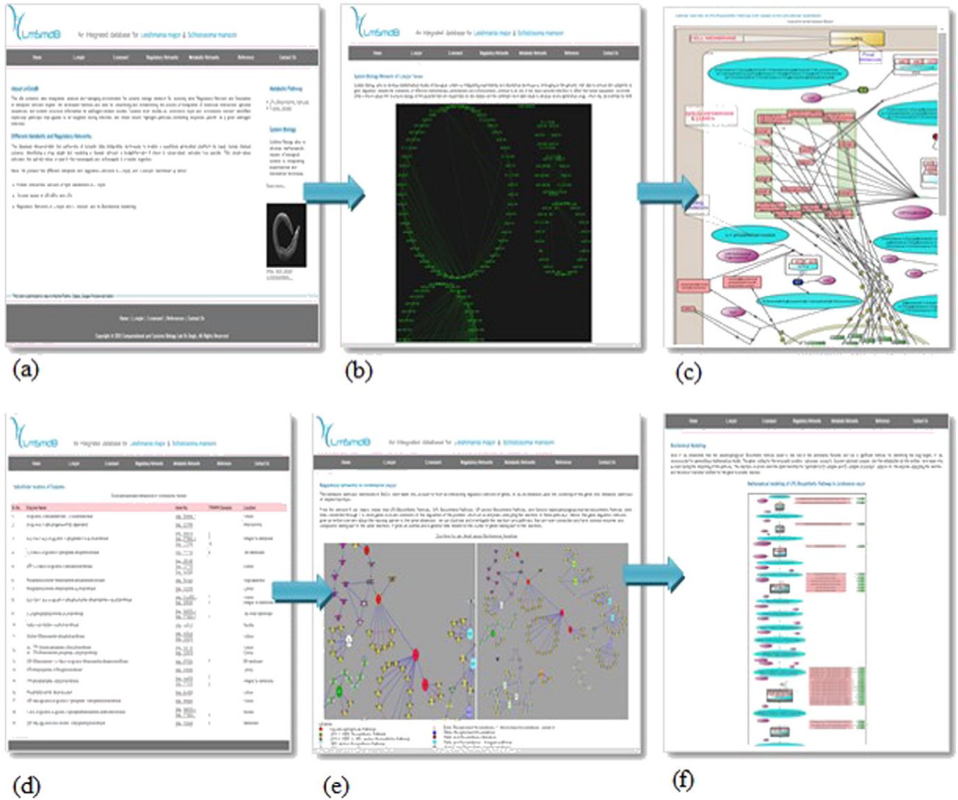
Fig. 2. LmSmdB database report page (a) home page of the database, gives information on the disease leishmaniasis and schistosomiasis, metabolic networks, regulatory networks, references and contact details. (b) GRN of Schistosoma mansoni . (c) Metabolic network reconstruction for L. major . (d) List of proteins in the network. (e) The Regulatory network of L. major . (f) The Metabolic network reconstruction in Schistosoma mansoni .
