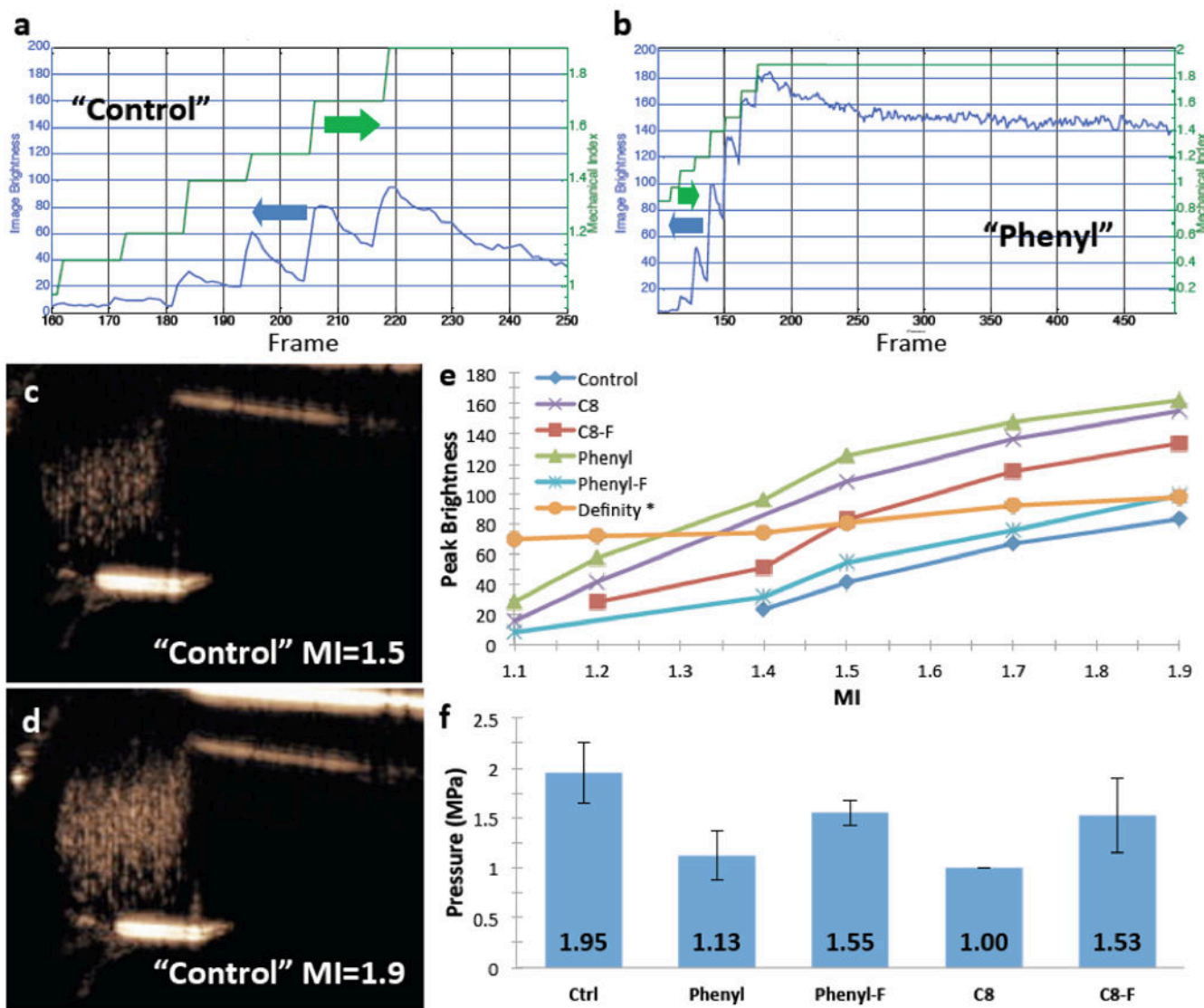
Figure 4. Image brightness over time with CPS imaging as a function of MI of PFP gas filled nanoshells
