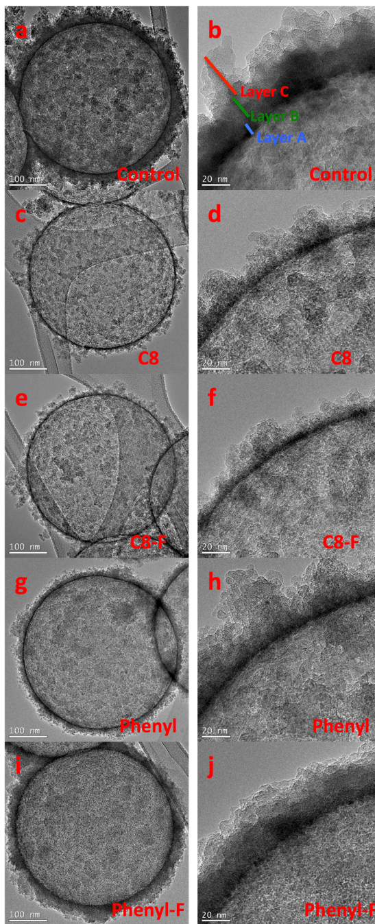
Figure 6. TEM images of all nanoshell formulations
