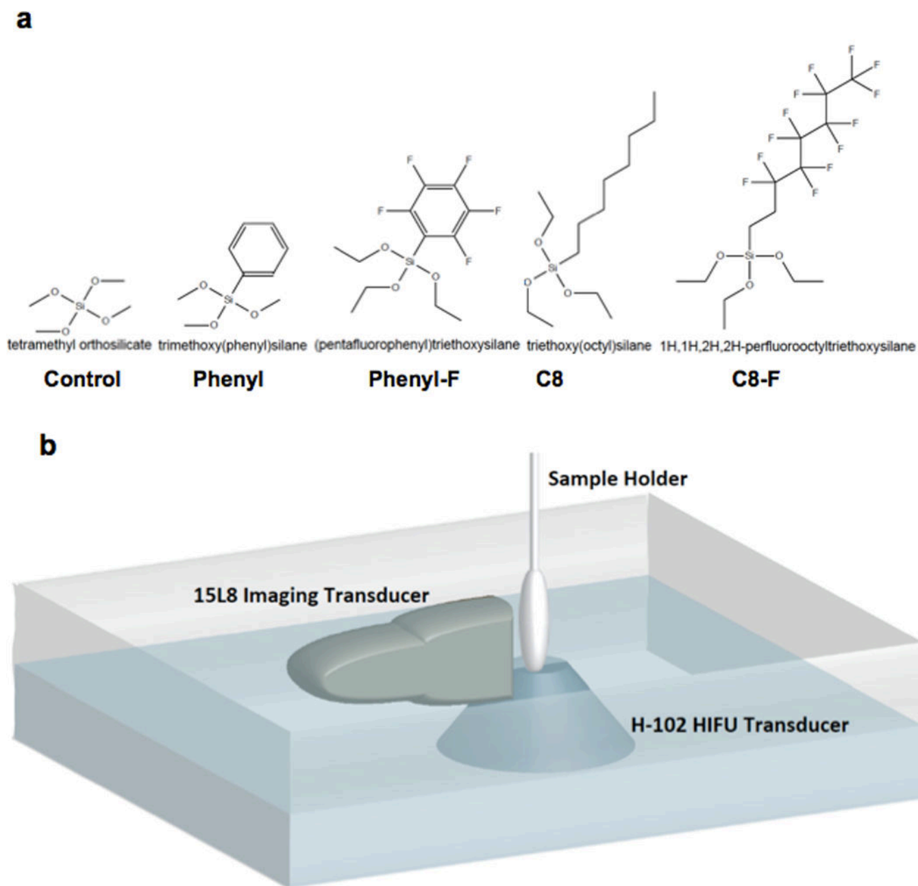
Figure 1. Structures of R-group substituted trialkoxysilanes and experimental set up for ultrasound testing of nanoshells
