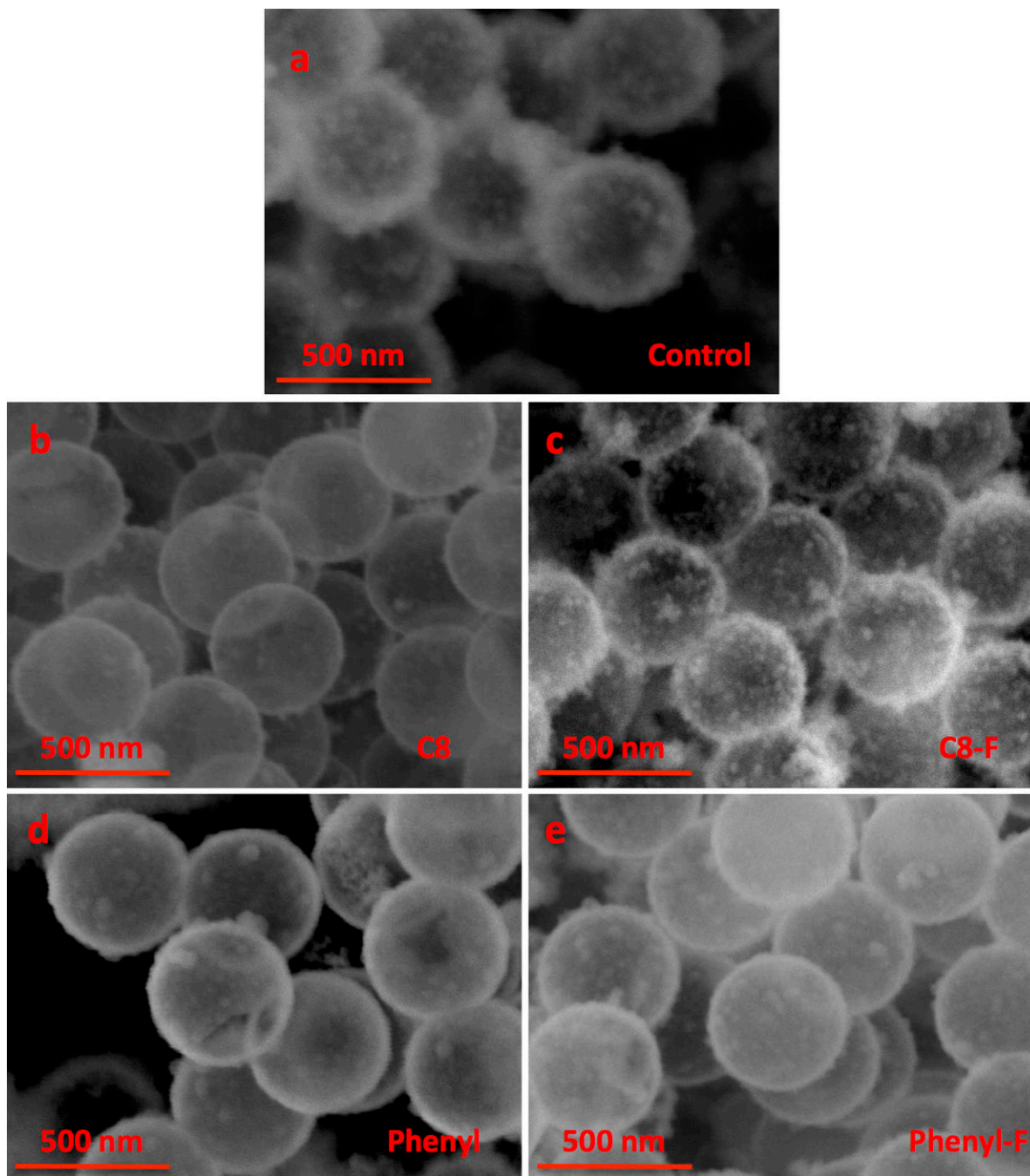
Figure 2. Scanning electron microscopy of various formulations at 74K Magnification after nanoshells have been calcined
