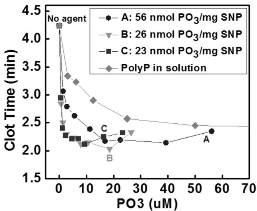
Figure 2. (Top) PolyP-SNP cuts clot time (R value using TEG) roughly in half versus SNP below 0.3 mg/ml. (Bottom) PolyP loaded onto silica lowers clot time compared to bare polyP when measured by fibrometry.
