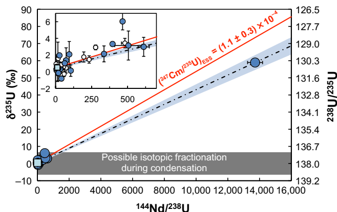
Fig. 1. \delta^{235}\text{U} plotted as a function of the ^{144}\text{Nd}/^{238}\text{U} ratio in meteoritic samples. Open circles, previous studies (11, 17–19, 33, 34); blue circles, Allende CAIs from this work; light-blue square, bulk Allende from this work]. The +59\text{‰} \delta^{235}\text{U} value observed in the Curious Marie CAI is well outside the range of variations expected from fractionation during condensation (gray rectangle) and is thus interpreted as definitive evidence for live ^{247}\text{Cm} in the ESS. The scatter in the data (for example, at very low Nd/U ratios) suggests that stable isotopic fractionation during evaporation/condensation also influenced the U isotopic composition of CAIs. The slope of the two-point isochron between Curious Marie and the rest of the samples translates into a ^{247}\text{Cm}/^{235}\text{U} of (0.9 \pm 0.07) \times 10^{-4} at the time of Nd/U fractionation in Curious Marie. Accounting for a possible delay between this fractionation event (possibly related to the extensive alteration of this CAI) and the formation of the SS of 5 \pm 5 My, the inferred ^{247}\text{Cm}/^{235}\text{U} at SS formation is (1.1 \pm 0.3) \times 10^{-4} (red line).
