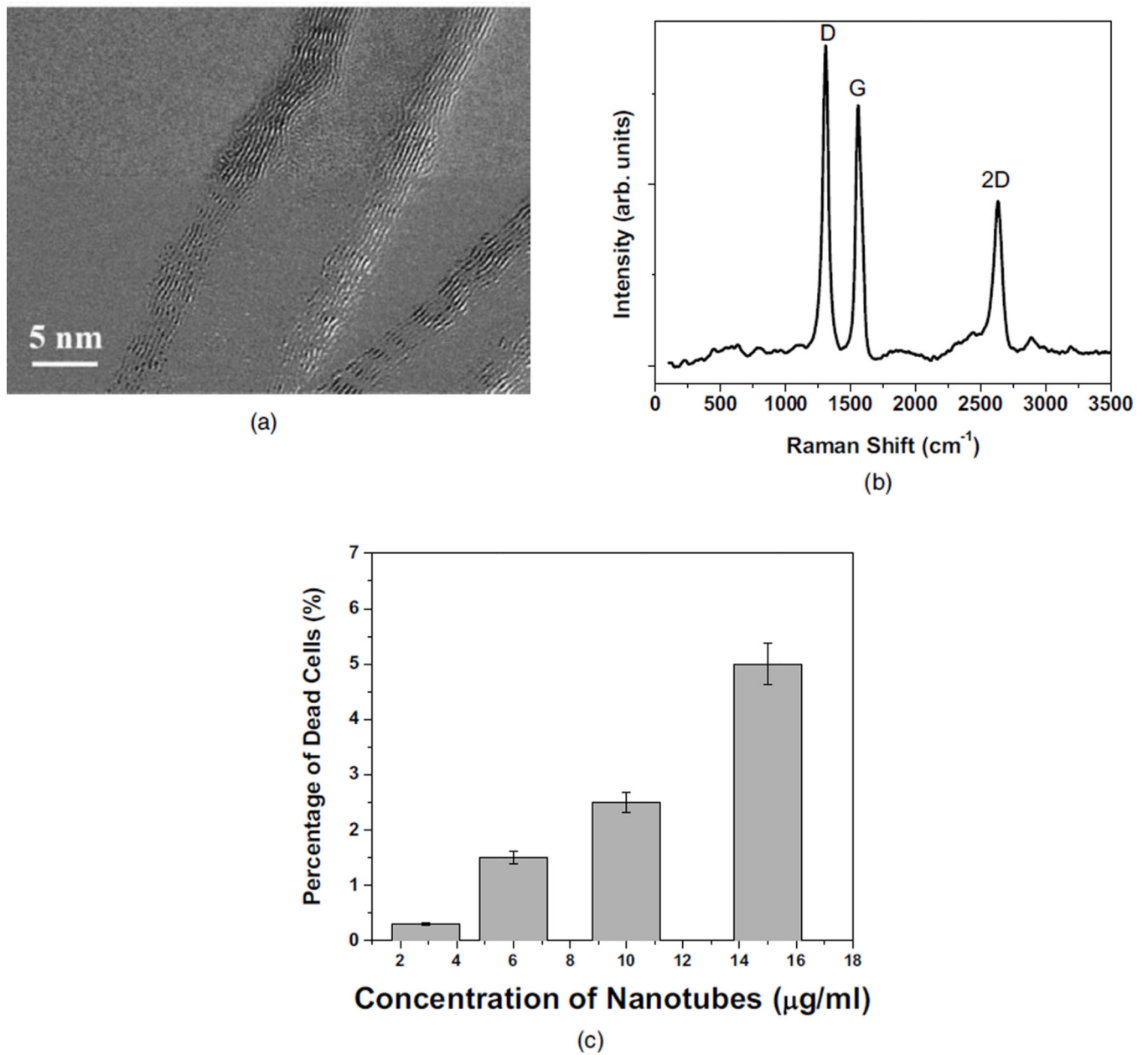
Fig. 2. High-resolution TEM image of multiwall CNTs (MWCNTs) grown over the Fe-Co/CaCO 3 catalyst, (b) Raman scattering spectra of the MWCNTs produced on the Fe-Co/CaCO 3 catalyst with acetylene as carbon source, and (c) cytotoxicity studies of the MWCNTs in the cervical cancer HeLa cells (48 h).
