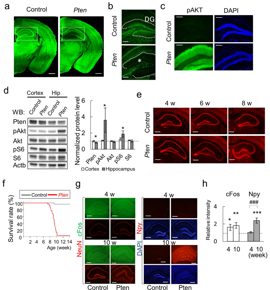
Figure 1. The characteristics and morphological findings of Pten -cKO mice. (a) Immunofluorescence studies on Pten expression (green). The left two panels show the coronary brain sections from control (left) and Pten -cKO (right, Pten ) mice at 4 weeks of age. The squares denote the areas of the hippocampus DG. Scale bar, 1 mm. (b) Confocal images with a higher magnification of the DG. Asterisk indicates the loss of Pten signals (green) in the granule cell layer of DG (dashed lines). Scale bar, 200 \mu m. (c) Hyperactive AKT signaling in the DG of Pten -cKO mice. The immunofluorescence signals of the phosphorylated S473 of AKT (pAKT, green) and DAPI (blue) are shown. Scale bar, 200 \mu m. (d) Western blotting of the cerebral cortex and hippocampal extracts from control and Pten -cKO mice at 8 weeks of age. The bar plots for the relative expression levels of the indicated proteins are shown in the right panel. Note that increased pAKT and pS6 signals are seen in the hippocampus, but not in the cerebral cortex of Pten -cKO. * P < 0.05 ( n = 4-6 , Wilcoxon rank sum test). (e) Progressive hypertrophy of the DG in Pten -cKO mice. The morphological changes of the DG hippocampal sections at the ages of 4, 6 and 8 weeks. See Supplementary Fig. S1 for the whole brain images. Scale bar, 500 \mu m. (f) Survival rates (%) of control and Pten -cKO mice. (g) cFos (green) and NeuN (red) expression (left panels). Npy (red) and DAPI (blue) expression (right panels), in the DG at 4 and 10 weeks of age. Scale bars, 500 \mu m. (h) The quantitated results of (f,g). The relative signal intensity ( Pten -cKO/control) of cFos and Npy at 4 and 10 weeks are plotted. Asterisks indicate significantly higher levels of cFos and Npy expressions in the DG of Pten -cKO mice in comparison to the control mice. P < 0.05 , ** P < 0.01 , ### and *** P < 0.001 ( n = 4-16 , Wilcoxon rank sum test).
