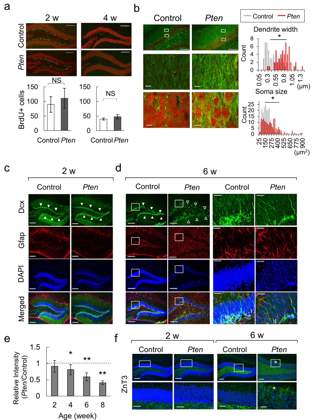
Figure 4. Hypertrophy of the DG and dysmorphic neurons in Pten -cKO mice. (a) BrdU (green) and NeuN (red) signals in the DG of the control and Pten -cKO mice at 2 and 4 weeks of age. The number of BrdU-positive cells in the subgranular zone are plotted (means \pm SD values, n = 3 ). NS, not significant. Scale bars (a–d) denote 200 \mu\text{m} unless otherwise stated. (b) Hypertrophy of the DG neurons in the Pten -cKO mice. Left images show Map2 (green) and NeuN (red) signals. Histograms represent the counts for indicated widths of dendritic shafts (right upper, 50 for control and 50 for Pten -cKO) and the sizes of soma (right lower, 200 control and 160 Pten -cKO) from 3 pairs of littermates are shown. *P < 0.0001 . Scale bars (lower panels), 10 \mu\text{m} . (c,d) Aberrant differentiation of neuronal progenitors in the DG of Pten -cKO. Dcx (green), Gfap (red) and DAPI (blue) signals are shown. Filled arrowheads indicate the Dcx signals peaked at the subgranular zone. Lucent arrowheads point to the sparse patterns of the Dcx signals at 6 weeks of age (d, Pten -cKO). Higher magnification views are provided for the boxed (d, far-right two columns). Scale bars, 20 \mu\text{m} (d) higher magnification images). (e) The relative fluorescence intensity ( Pten -cKO/control) of Dcx in the subgranular zone at 2, 4, 6 and 8 weeks of age (mean \pm SD, n \geq 3 ). (f) Znt3 (green) and DAPI (blue) signals in DG at 2 and 6 weeks of age. Asterisks indicate the presence of abnormal sprouting of mossy fibers. The lower panels show higher magnification views of the boxed areas. Scale bars, 50 \mu\text{m} (lower panels).
