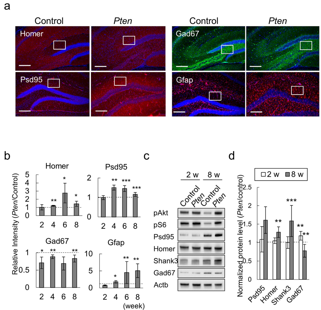
Figure 3. Excitatory-inhibitory imbalance in the hippocampus of Pten -cKO mice. (a) The expression of excitatory synapse (Homer, Psd95), inhibitory neuron (Gad67) and glial markers (Gfap) in the hippocampus of control and Pten -cKO mice at 6 weeks of age. Immuno-labeled proteins are annotated. Squares indicate the ROIs for the quantitative analyses. Scale bar, 200 \mu m. (b) The quantitated results of the immunofluorescence studies. The relative fluorescence intensity ( Pten -cKO/Control) of Homer, Psd95, Gad67 and Gfap are plotted for 3 or more independent pairs of Pten -cKO and control littermates at each time point. Horizontal dashed lines indicate the reference values of the control mice. (c) Representative images of western blots for the hippocampal extracts. Three or more pairs of control and Pten -cKO mice at 2 and 8 weeks of age were used for this study. (d) The quantitated Western blotting data. Bar plots for the relative expression ( Pten -cKO/Control) of the indicated proteins. The plotted values show the means \pm SD ( n \geq 3 ). In panels (b,d), * P < 0.05 , ** P < 0.01 , *** P < 0.001 .
