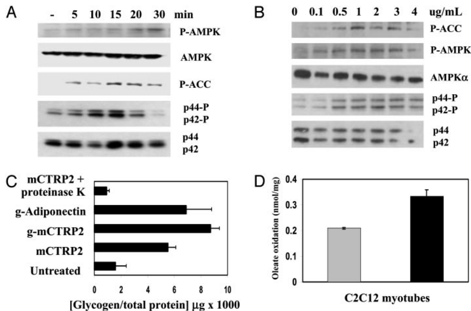
Fig. 5. Effects of mCTRP2 on C2C12 myotubes. (A) Differentiated C2C12 myotubes were untreated or treated with 4 \mu\text{g/ml} of recombinant mCTRP2 for 5, 10, 15, 20, and 30 min. Western blot analyses were carried out on cleared cell lysates by using antibodies specific for phospho-ACC (Ser-79), phospho-AMPK (Thr 172), total AMPK- \alpha , phospho-p44/42 MAPK (Thr-202/Tyr-204), and total p44/42 MAPK. (B) Differentiated C2C12 myotubes were stimulated with recombinant mCTRP2 proteins (0–4 \mu\text{g/ml} ) for 15 min, and Western blot analyses were carried out on these cell lysates. (C) Differentiated C2C12 myocytes were treated for 16 h with 4 \mu\text{g/ml} of recombinant g-adiponectin (globular domain only; positive control), CTRP2 (full-length), gCTRP2 (globular domain only), or mCTRP2 predigested with proteinase K. The amount of glycogen in these cells was determined and normalized to total cellular protein. (D) [ ^{14}\text{C} ]oleate oxidation was measured in differentiated C2C12 myotubes. The formation of ^{14}\text{CO}_2 was determined in cells incubated for 90 min in the absence (gray) or presence (black) of 4 \mu\text{g/ml} mCTRP2. Incubation with mCTRP2 led to a statistically significant increase in oleate oxidation ( P = 0.0023 , Student's t test). Each experiment was performed in triplicate.
