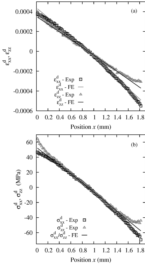
Figure 11 (a) Profile of the deviatoric strain components \varepsilon_{xx}^d and \varepsilon_{zz}^d and (b) profile of the deviatoric stress components \sigma_{xx}^d and \sigma_{zz}^d , obtained by the Laue-DIC method on a Si single-crystal during bending at 50 N. In (b), the line referring to as 'FE' is the finite-element results for \sigma_{xx}^d and \sigma_{zz}^d .
