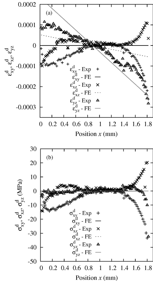
Figure 12 (a) Profile of the shear strain components \varepsilon_{xy}^d , \varepsilon_{xz}^d and \varepsilon_{yz}^d and (b) profile of the shear stress components \sigma_{xy}^d , \sigma_{xz}^d and \sigma_{yz}^d obtained by the Laue-DIC method for the Si single-crystal. Case 50 N.
