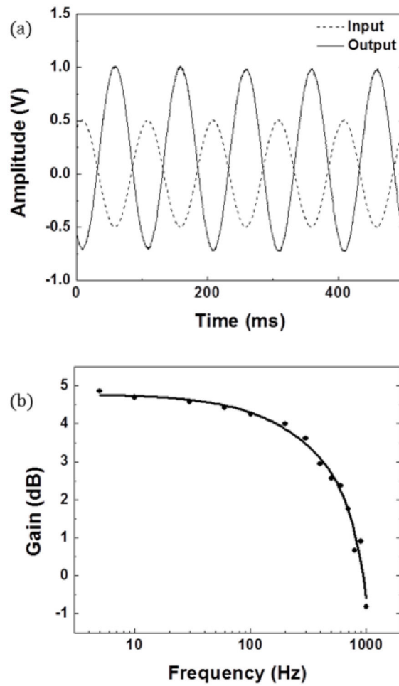
Fig. 3. Results from common source amplifier using pentacene TFT showing the (a) representative output versus input and (b) bode plot. Both results shown were taken from the same 100 \mu m channel length device.
