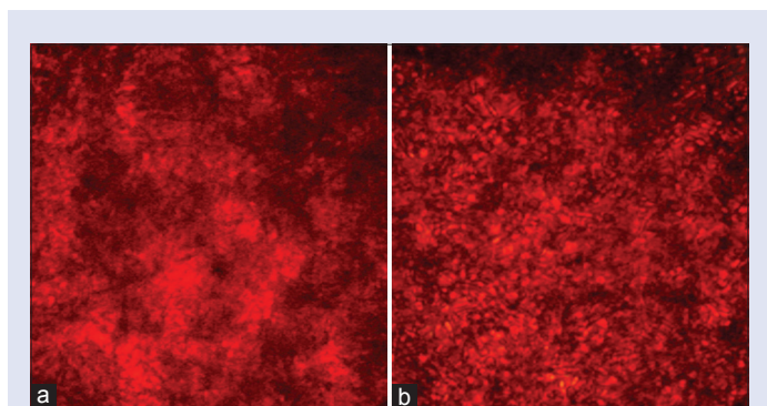
Figure 1: Effect of 7-hydroxycalamenene against Candida albicans biofilm. The plates were incubated at 37°C for 24 h. (a) Biofilm control, (b) Biofilm treated with 2500 µg/ml of 7-hydroxycalamenene. The images were taken at ×40 using an inverted microscope
