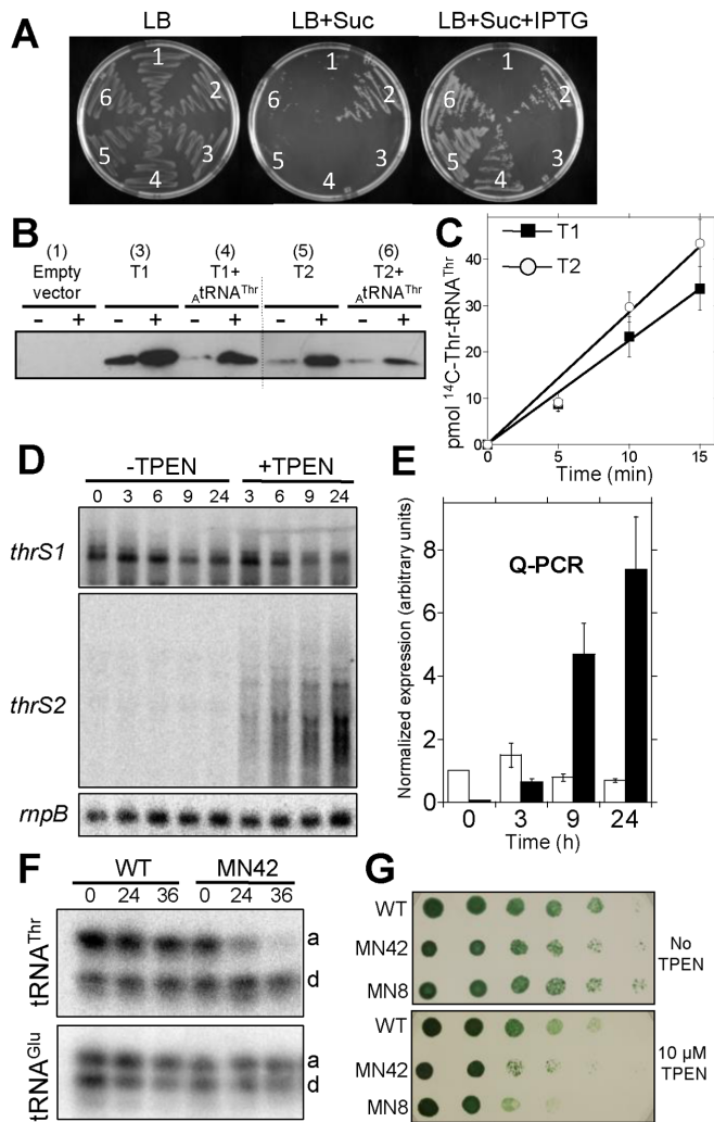
Figure 1. Functional characterization of T1 and T2. (A) Complementation assay of the E. coli conditional mutant IBPC6881(pSGUB4). Derived strains containing the empty vector pTrc99A (sector 1) or derived plasmids expressing the E. coli ThrRS (sector 2), T1 (sector 3), T1 and Anabaena tRNA Thr (CGU) (sector 4), T2 (sector 5), T2 and Anabaena tRNA Thr (CGU) (sector 6) were streaked on the indicated media. (B) Lack of complementation is not due to a deficient expression of T1 in E. coli . Western blot of extracts were carried out using 10 μg protein extracts from the strains used in the complementation assay that express the indicated products, cultured (+) or not (-) with 1 mM IPTG and incubating with anti-hexahistidine antibodies. Numbers indicate the corresponding sector for each strain in the complementation assay. (C) Aminoacylation assay with recombinant T1 or T2 proteins. Assays were carried out in a volume of 22 μl and contained 50 nmol of T1 or T2 and 5 μM Anabaena tRNA Thr (CGU). Average values ± s.d. of three independent experiments are represented. (D) Northern blot with RNA from Anabaena cells subjected or not to incubation in the presence of chelating agent TPEN for the indicated period of time (in hours). Genes used as probes are indicated. (Northern assays of thrS2 in these conditions have been published elsewhere (38), and it is only shown here for the sake of comparison). (E) Quantitative Real-Time PCR analysis of transcripts of thrS1 and thrS2 from cells incubated or not with 20 μM TPEN for the time indicated in hours in the horizontal axis. Levels of the thrS1 gene in cells not incubated with TPEN (t = 0) were assigned the arbitrary value of 1 and all other measures were expressed in proportion to this value. Empty and solid bars correspond to thrS1 and thrS2 , respectively. Average values ± SE of three independent biological replicas are represented. (F) Total tRNA (2 μg) from WT Anabaena cells or the deletion mutant MN42 ( \Delta thrS2 ) cultured for the indicated time (in hours) in the presence of 20 μM TPEN were re-
