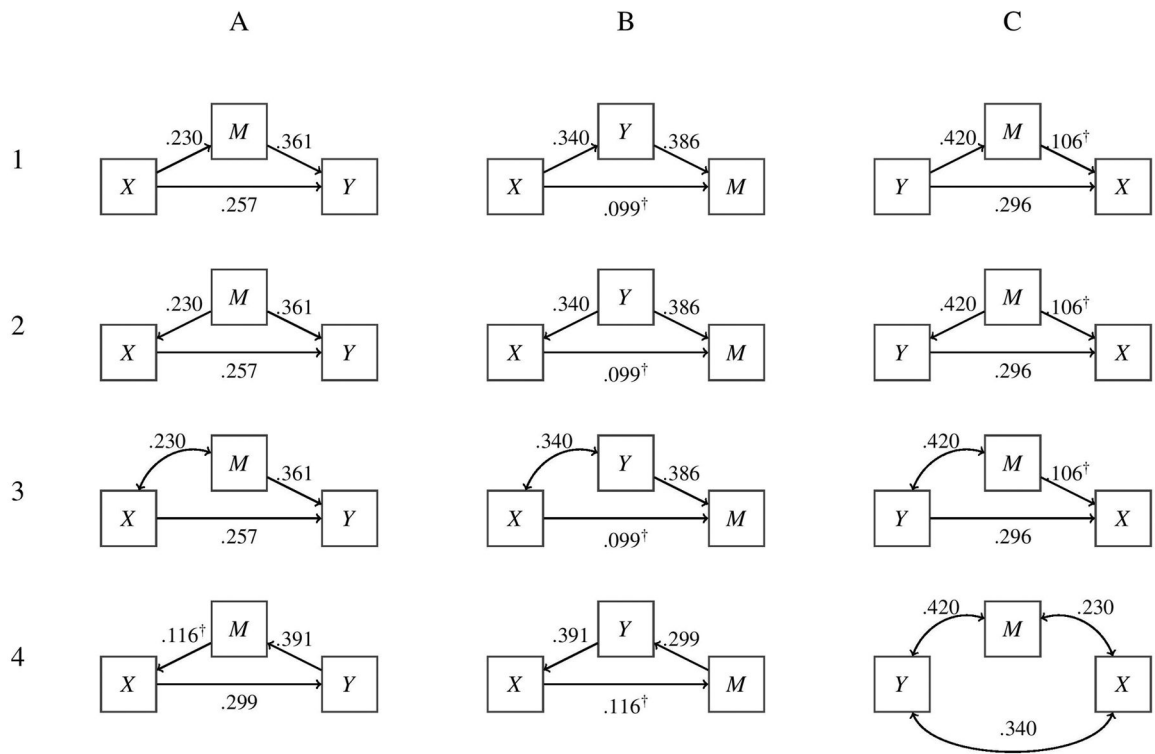
Figure 2. The set of 12 plausible equivalent models associated with the simple mediation model reported in Garcia et al. (2012). X = persistence, M = self-directedness, and Y = positive affect. All standardized path coefficients and Person correlation coefficients, situated above nondirectional pathways, are significant at \alpha = .05 unless indicated by
