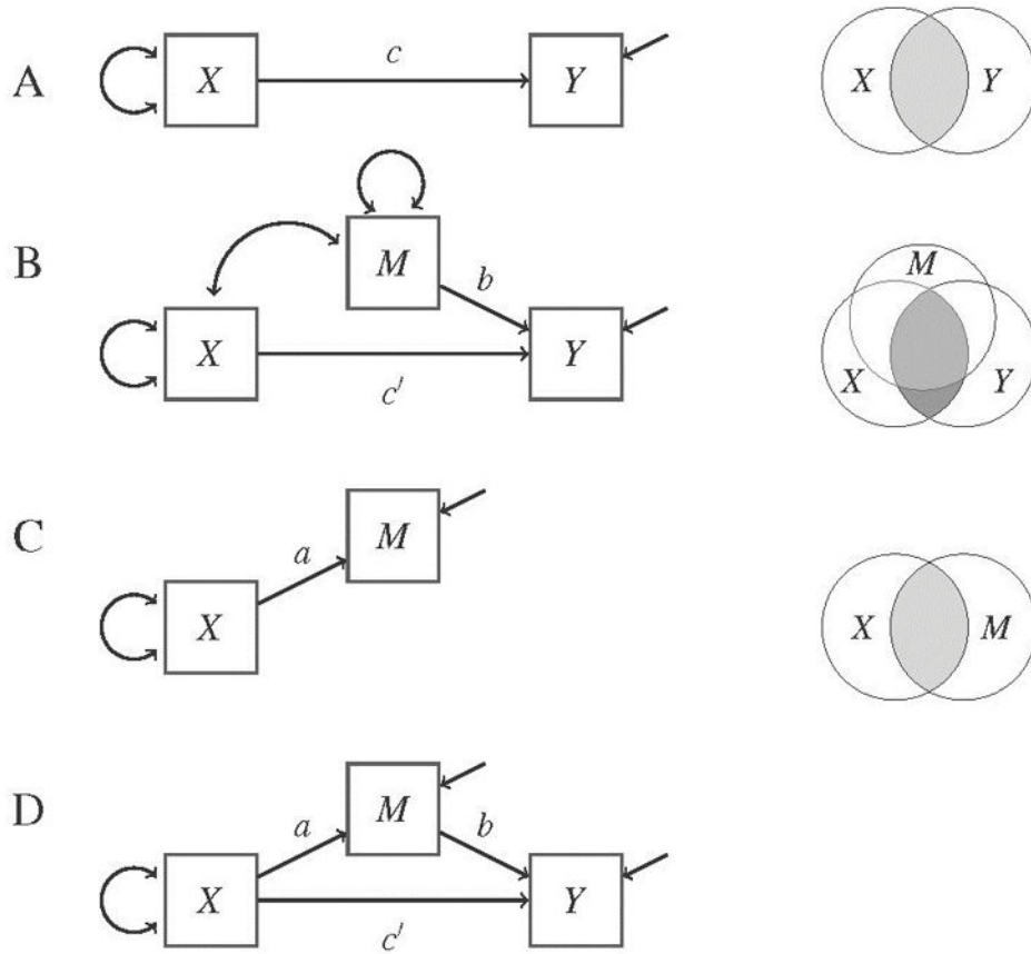
Figure 1. Four sets of diagrams depicting concepts in mediation. Diagrams on the left are path diagrams with letters a , b , c and c' representing standardized coefficients. Diagrams on the right are Venn diagrams where the shaded areas between circles relate to shared variances among the variables. Endogenous variables with arrows pointing towards them are dependent variables and exogenous variables with arrow emerging from them are independent variables.
