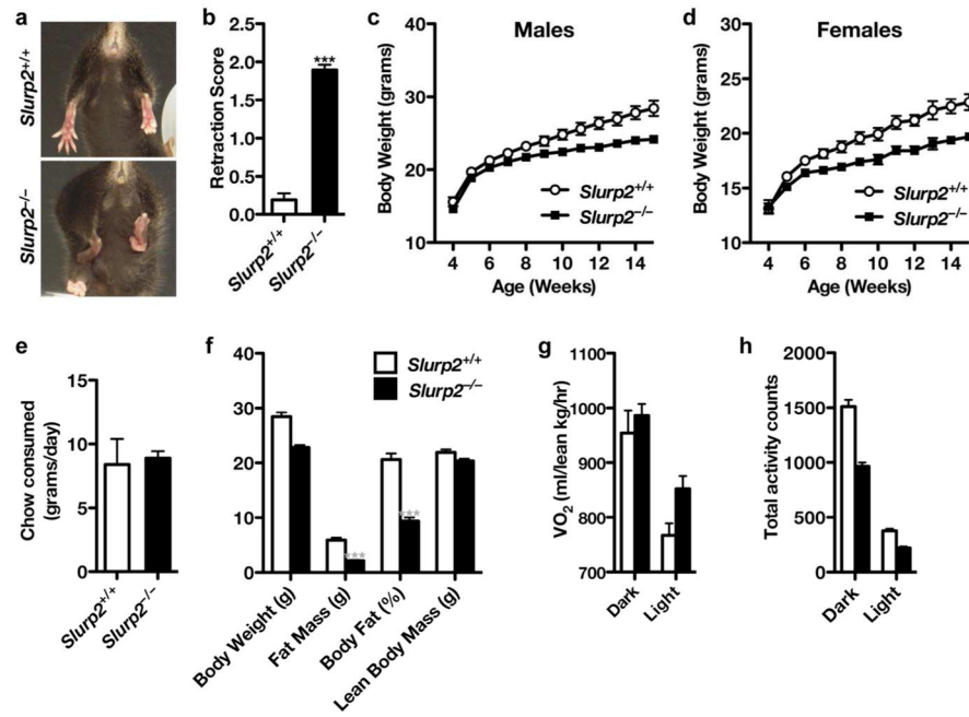
Figure 2. “Non-skin” phenotypes in Slurp2 -/- mice
