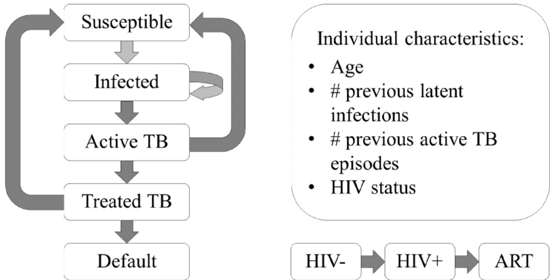
Figure 1. Model structure
