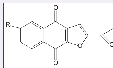
Figure 9a: Naphtho [2,3-b] furan-4,9-dione
