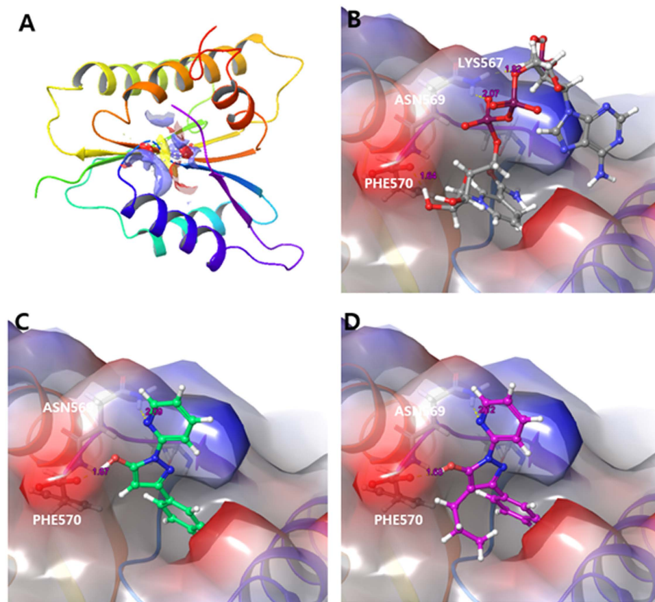
Figure 2. (A) Determination of docking site of crystal structure of NADPH binding domain of gp91 phox (PDB ID: 3A1F). (B) NADPH was bound the NADPH binding domain of gp91 phox . (C) Ewha-89403 (Green) was bound the NADPH binding domain of gp91 phox . (D) Ewha-18278 (purple) was bound the NADPH binding domain of gp91 phox .
