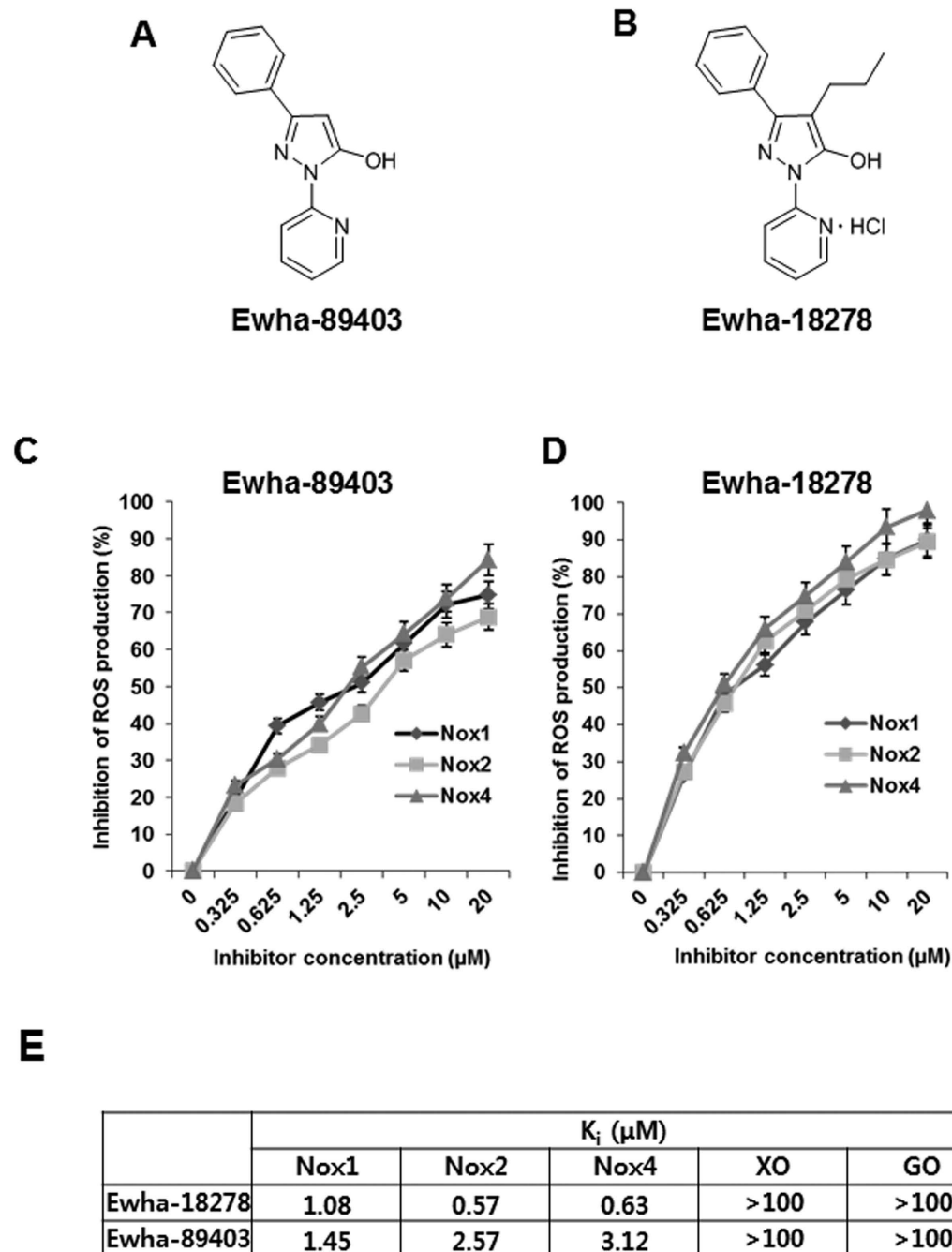
Figure 1. Chemical structure and Nox inhibition profile of Ewha-89403 and Ewha-18278. (A) Chemical structure of Ewha-89403. (B) Chemical structure of Ewha-18278. (C,D) Concentration-dependent Nox inhibition curves of Ewha-89403 (C) and Ewha-18278 (D). Drosophila membranes specifically overexpressing hNox1, hNox2, and hNox4 were subjected into ROS measurement with Diogene. (E) K_i value of Ewha-89403 and Ewha-18278 on hNox1, hNox2, hNox4, xanthine oxidase (XO) and glucose oxidase (GO).
