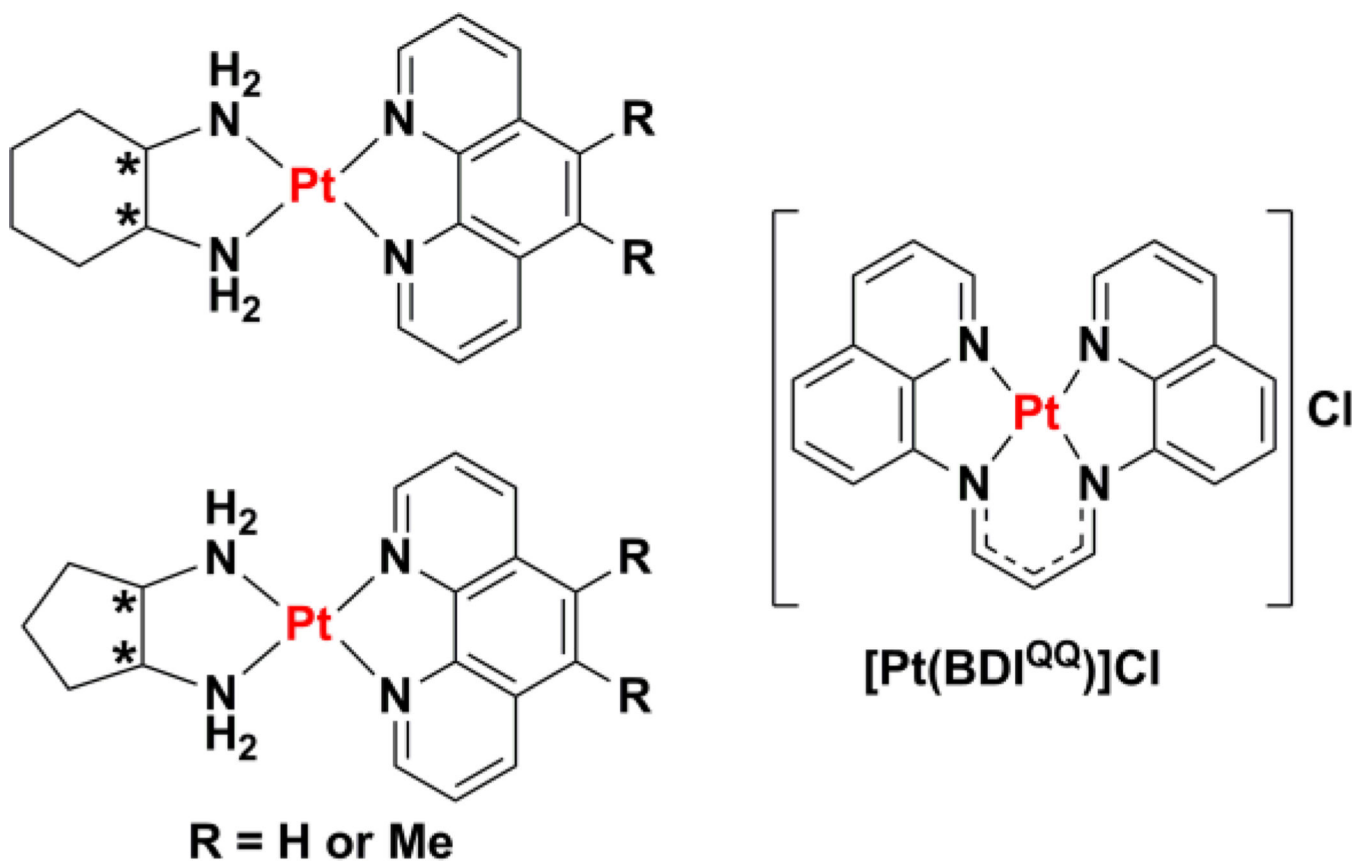
Chart 11. Chemical structure of platinum(II) complexes that bind to DNA through non-covalent interactions.
